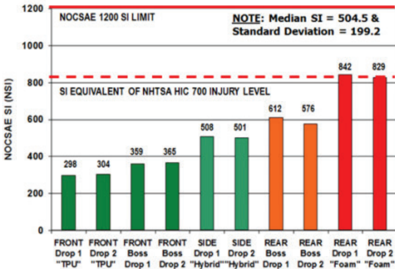
Fig-2. NOCSAE Severity Index Data from 2014 Peewee Youth Helmet Design Approved for Peewee Play
