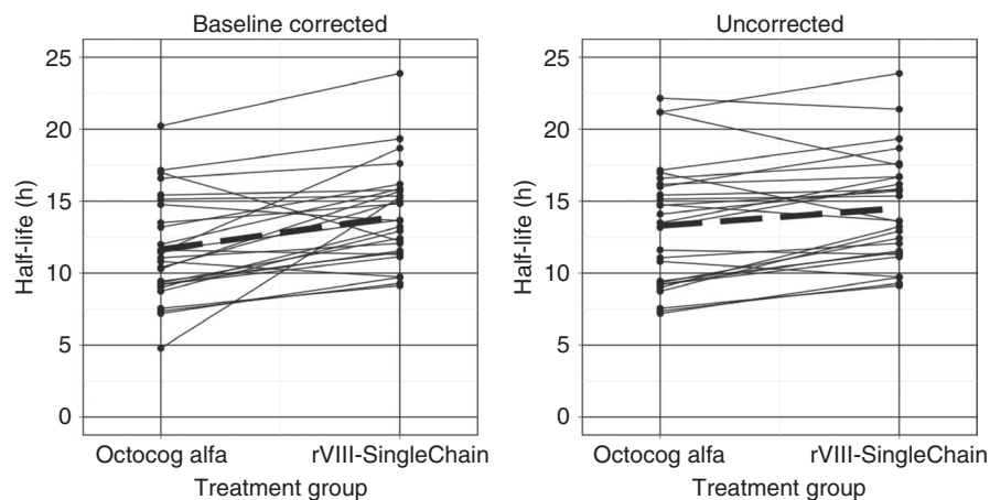
FIGURE 3 Example of individual PK parameters after switching
