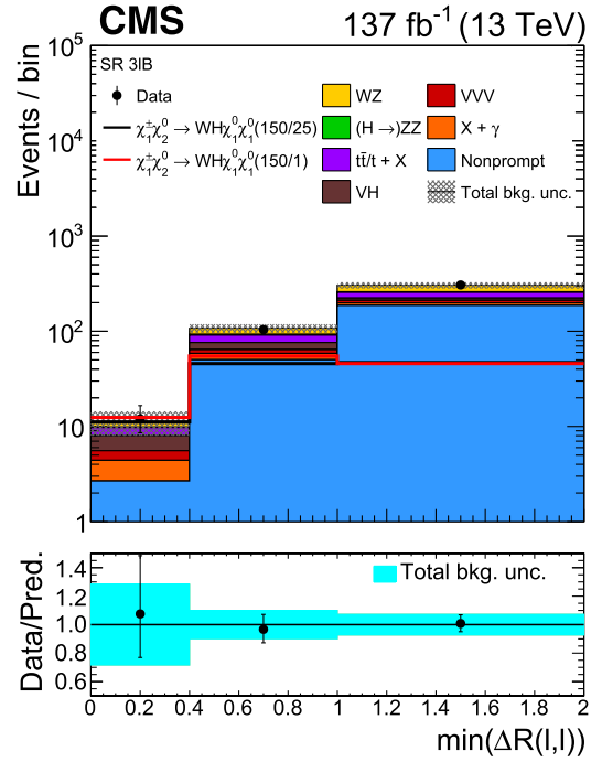
FIG. 10. “ 2S\ell/\geq 3\ell ” search: observed and expected event yields across the SRs in category B, events with three light leptons and no OSSF pair, after the requirement that the leading-lepton p_T be greater than 30 GeV is applied. The prefit signal distributions for two mass-points are overlaid for illustration, and the considered mass hypothesis is indicated in the legend with notation [m(\text{NLSP})/m(\text{LSP})] ; for example (150/1) stands for m_{\tilde{\chi}_1^\pm} = m_{\tilde{\chi}_2^0} = 150 GeV, m_{\tilde{\chi}_0} = 1 GeV. “Nonprompt” refers to the background contribution arising from nonprompt or misidentified leptons.
