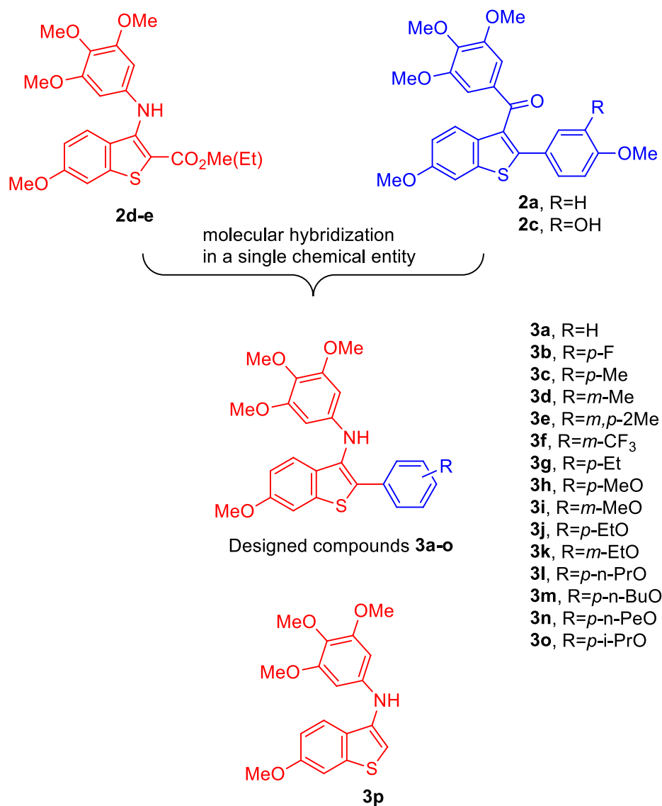
Figure 2. Design strategy for conjugates 3a-p obtained by the combination of pharmacophores of compounds 2a and 2c-e .
