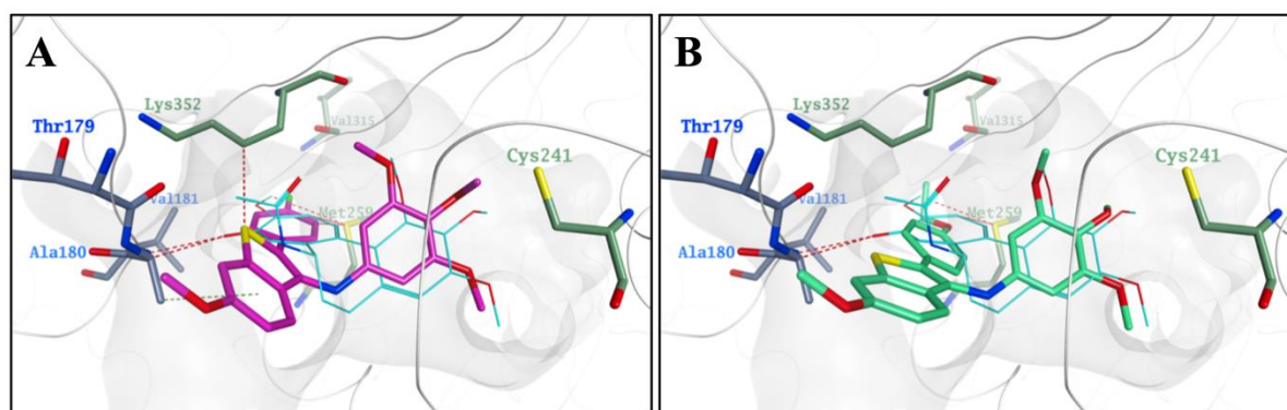
Figure 3. A) Proposed binding for compound 3b in the colchicine site. The trimethoxyphenyl ring is in proximity to \beta Cys241, while the benzo[ b ]thiophene portion is pointing towards the tubulin \alpha -subunit. The p -fluoro phenyl ring is placed in a small hydrophobic area near
