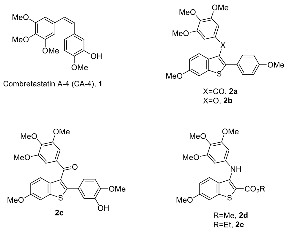
Figure 1. Chemical structure of CA-4 ( 1 ) and representative examples of benzo[ b ]thiophene derivatives ( 2a-e ).
