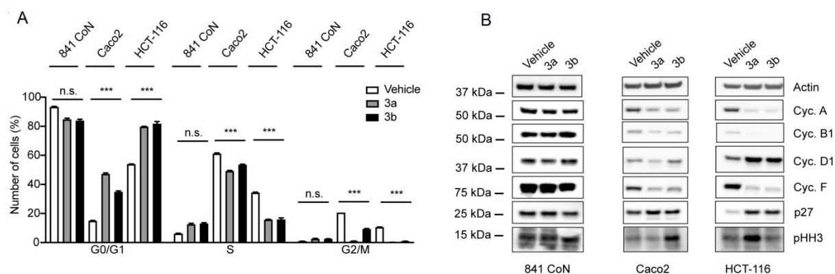
Figure 5. (A) Calculation in percentage of the amount of 841 CoN, Caco2 and HCT-116 cells in G0/G1, S and G2/M phases in basal condition and after 3a (grey bar) or 3b (black bar) treatments at 60 or 400 nM, respectively, on the basis of the PI uptake. (B) Cell cycle marker investigation under the same conditions as were used in Panel A by using selective antibodies against markers of the cell cycle: Cyc. D1 and p27 for G1 phase; Cyc. A for S phase; Cyc. F and B1 for G2/M; pHH3 for mitosis. Cyc. = Cyclin; n.s. = not significant; *** = p < 0.001 .
