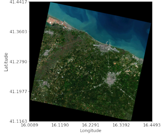
Figure 2: A PRISMA image in RGB channels acquired on 05/12/2022.
