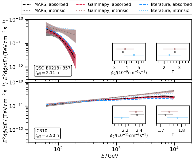
Fig. 8. SEDs of QSO B0218+357 (top) and IC310 (bottom). Lighter colours represent the estimated spectra without the effect of the EBL absorption. The inlets represent the estimated spectral parameters.
