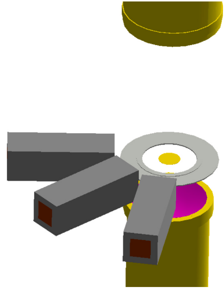
Fig. 16. A schematic view of the setup simulated in Geant4 with three sTED modules and the gold sample.
