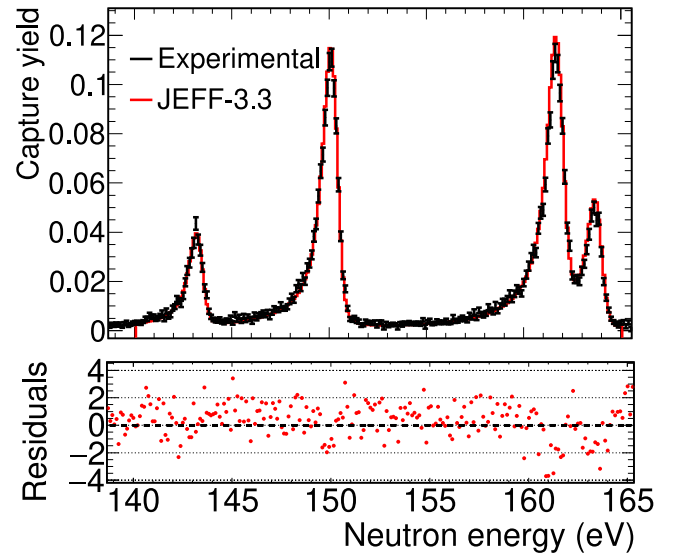
Fig. 21. sTED experimental capture yield obtained with a ^{197}\text{Au} sample (Experimental) compared with the yield obtained from the JEFF-3.3 nuclear data library (JEFF-3.3) in the energy region between 140 and 165 eV. In the bottom panel of the figure, the residuals defined as the distances of the experimental data points to the theoretical JEFF-3.3 yield divided by the statistical uncertainties of the data points are plotted. The error bars consider only the uncertainties due to counting statistics.
