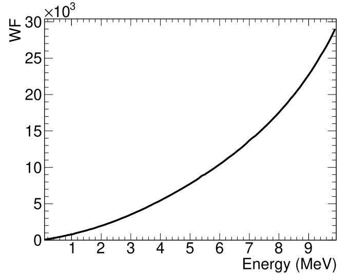
Fig. 17. Adopted WF for one sTED module. WF(E) = 6.5071 + 656.261 \cdot E + 113.929 \cdot E^2 + 34.5488 \cdot E^3 - 6.39125 \cdot E^4 + 0.411521 \cdot E^5 , the energy ( E ) is given in MeV and the coefficients correspond to k = 1 , see 3.3.
