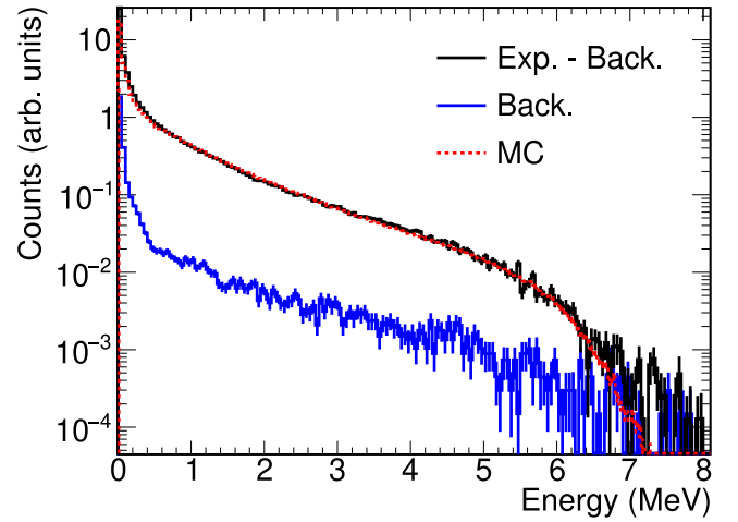
Fig. 20. Experimental deposited energy spectra in one sTED module (Exp.-Back.) with background (Back.) subtracted and simulated with Geant4 (MC) for ^{197}\text{Au} (n, \gamma ) cascades.
