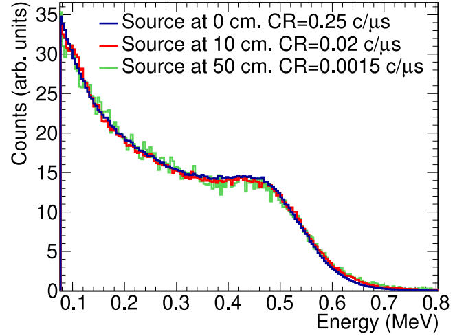
Fig. 12. Deposited energy spectra for a 20 MBq 137 Cs calibration source placed at different distances from an sTED module with an R11265U-100 photomultiplier, along with the Counting Rates (CR) obtained using a deposited energy threshold of 0.15 MeV.
