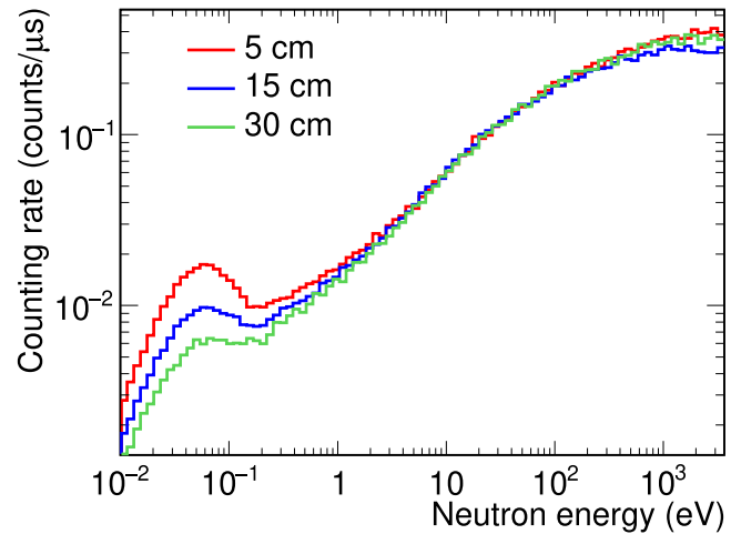
Fig. 2. Counting rates obtained for a BICRON detector as a function of the neutron energy with a 0.15 MeV deposited energy threshold in a beam-on measurement without any sample in place at the nominal proton intensity. The measurements are performed with the detector at the same distance from the spallation target but at three different distances (5, 15 and 30 cm) from the center of the beam.
