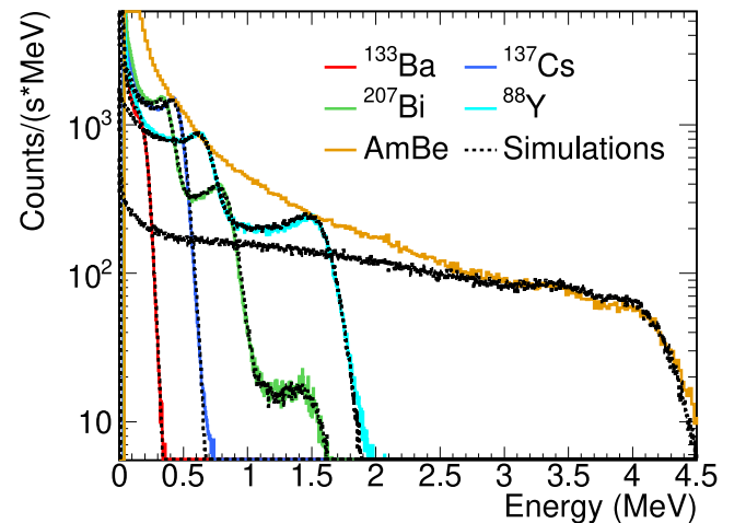
Fig. 14. Experimental deposited energy spectra obtained with an sTED module for various \gamma -ray sources ( ^{133}\text{Ba} , ^{137}\text{Cs} , ^{207}\text{Bi} , ^{88}\text{Y} and AmBe) compared with Geant4 simulations. The area of the experimental spectra are normalized to the simulated ones.
