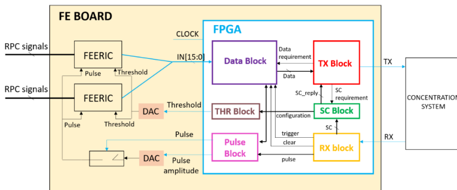
Figure 7. Block diagram of the front-end board for SHiP RPCs.
