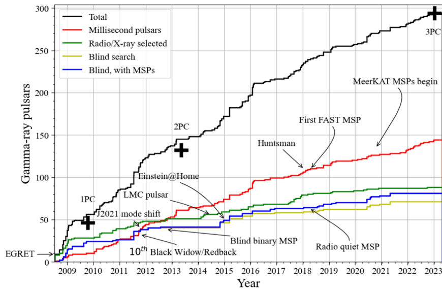
Figure 1. Cumulative number of known gamma-ray pulsars, beginning with the launch of Fermi. The crosses show the numbers included in the first (IPC) and second (2PC) catalogs of LAT pulsars and their publication dates. Some key discoveries are highlighted. See also Table 1.
