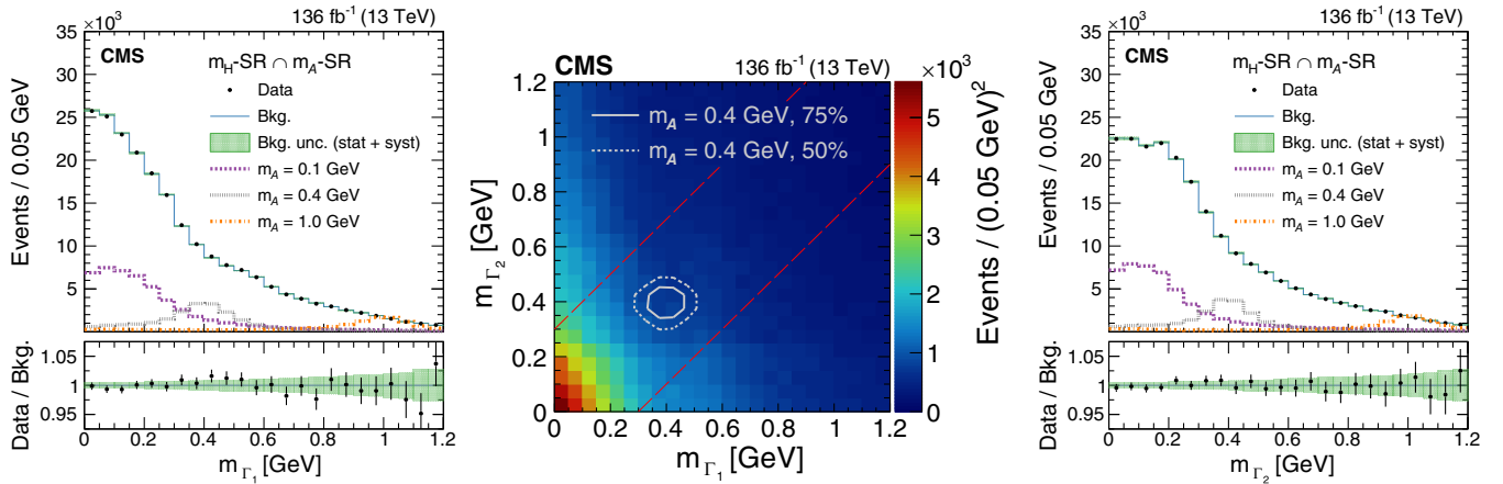
FIG. 1. Mass distributions from selected events in data. Center: the 2D-m_\Gamma distribution for data events in the m_H -SR. The red dashed lines indicate the m_A -SR boundaries. The contours of simulated H \rightarrow \mathcal{A}\mathcal{A} \rightarrow 4\gamma events for m_A = 0.4 GeV are plotted for 75% (solid contour) and 50% (dotted contour) of the distribution maximum. The corresponding m_{\Gamma_1} (left) and m_{\Gamma_2} (right) projections for the overlap of the m_H -SR and m_A -SR are also shown. The data distributions (black points) are plotted against the total predicted background distributions (blue curves). The statistical uncertainties in the former are negligible and the total uncertainties in the latter are barely visible as green bands. The spectra of simulated H \rightarrow \mathcal{A}\mathcal{A} \rightarrow 4\gamma events for m_A = 0.1 (purple dashed curve), 0.4 (gray dotted curve), and 1.0 GeV (orange dash-dotted curve) are also provided. They are each normalized to the value of \mathcal{B}(H \rightarrow \mathcal{A}\mathcal{A} \rightarrow 4\gamma) that is expected to be excluded by the background model (described under the CL_s criterion in our results) times 10^3 . The black points in the lower panels of the left and right plots give the ratios of the data to the predicted background distributions. The vertical bars represent the statistical uncertainties in the former, and the green bands represent the total uncertainty in the latter.
