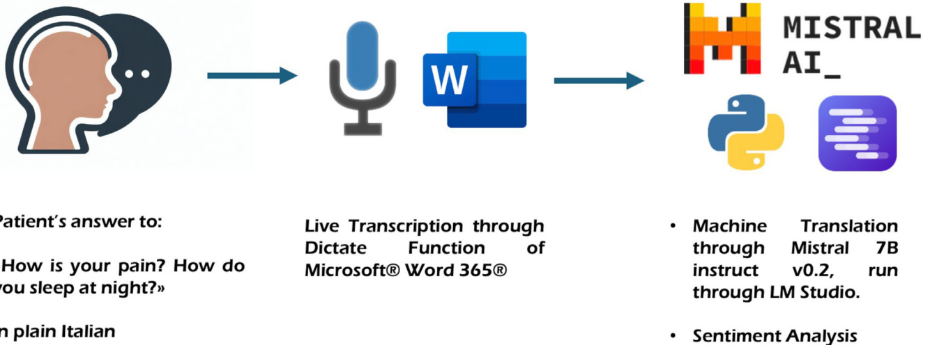
Figure 1 Workflow for sentiment analysis.
