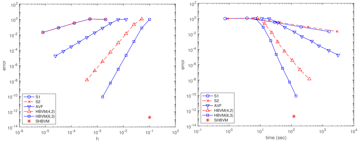
Fig. 2. Example 1 - error versus stepsize (left-plot) and error versus execution time (right-plot).
