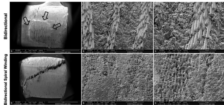
Figure 2. Representative scanning electron microscopy photos of bFRC and bswFRC fractures at different magnifications (×31, ×500 and ×1000). Black arrows indicate a shear fracture in bFRC sample.
