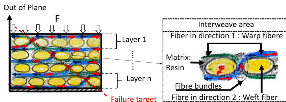
Figure 4. Illustration of out-of-plane compression failure mechanism of woven fibre composite. Red \rightarrow arrow and blue \leftarrow arrow: local normal forces transferred to fibre due to Poisson effect. \nearrow Double red arrow: Forces in fiber bundles zone which is a combination of shear, tensile and compression forces. \downarrow Black arrow: compression-loading force. Dash red line: Failure target. For bswFRC, the mechanical stress concentration is in interweave zone (bundle zone). Thus, the failure target across this bundle zone.
