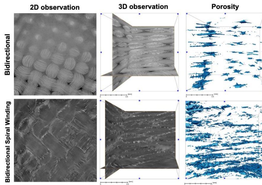
Figure 3. Volume rendering of the segmented pores (blue color) in bFRC and bswFRC, obtained by X-ray tomography analysis. The scale bar corresponds to 0.5 mm in all images.
