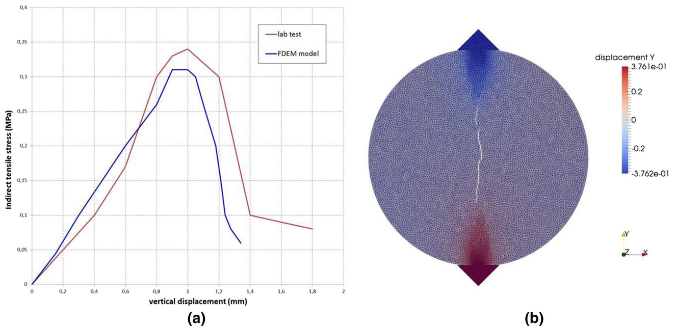
Fig. 11 a Indirect tension test simulation on a calcarenite sample performed with FDEM Irazu software compared with laboratory data; b vertical displacement and failure mode obtained from the FDEM test simulation
