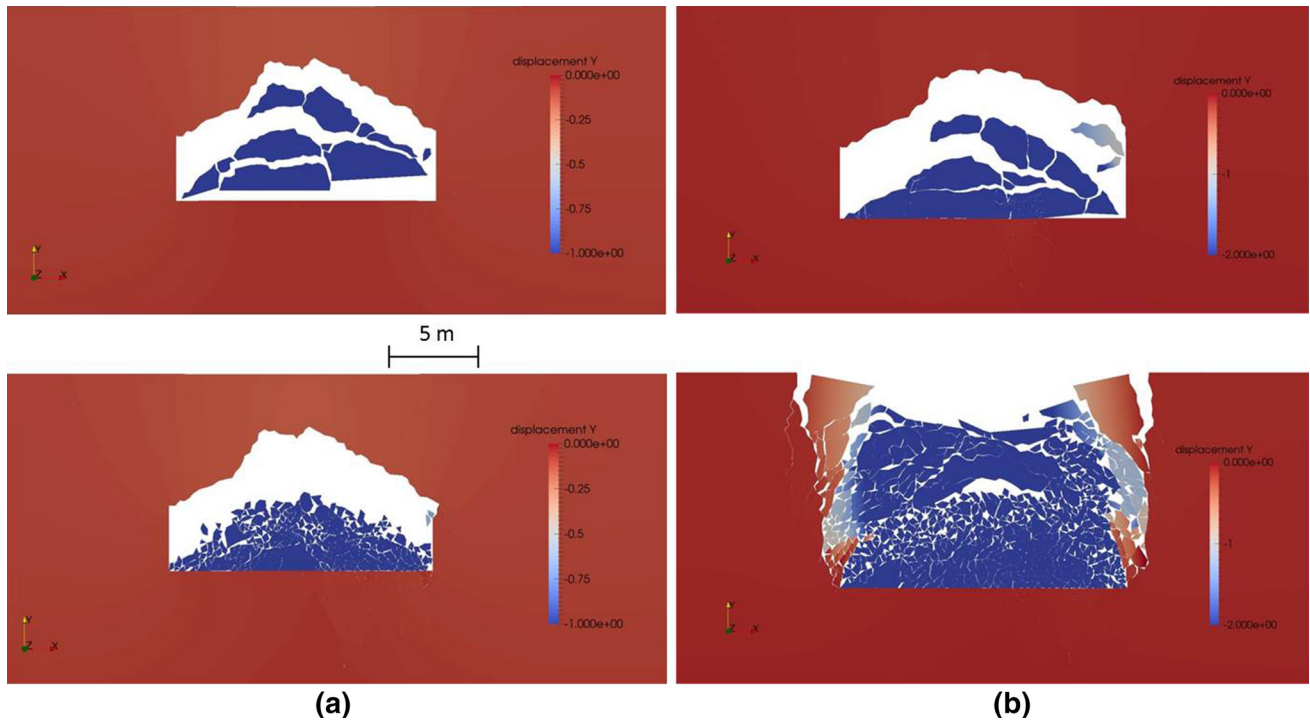
Fig. 18 16 \times 4 m cavity FDEM model: vertical displacements obtained with a G_{If} = 20 N/m– G_{III_f} = 200 N/m fracture energy parameters; b G_{If} = 10 N/m– G_{III_f} = 100 N/m fracture energy parameters
