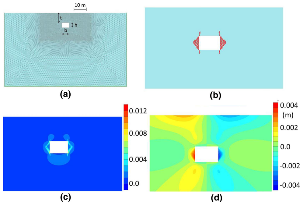
Fig. 13 FEM model of the 6 \times 4 \text{ m} underground cavity: a FEM discretization mesh and geometrical parameters, b plastic points, c deviatoric strains, d horizontal displacements
