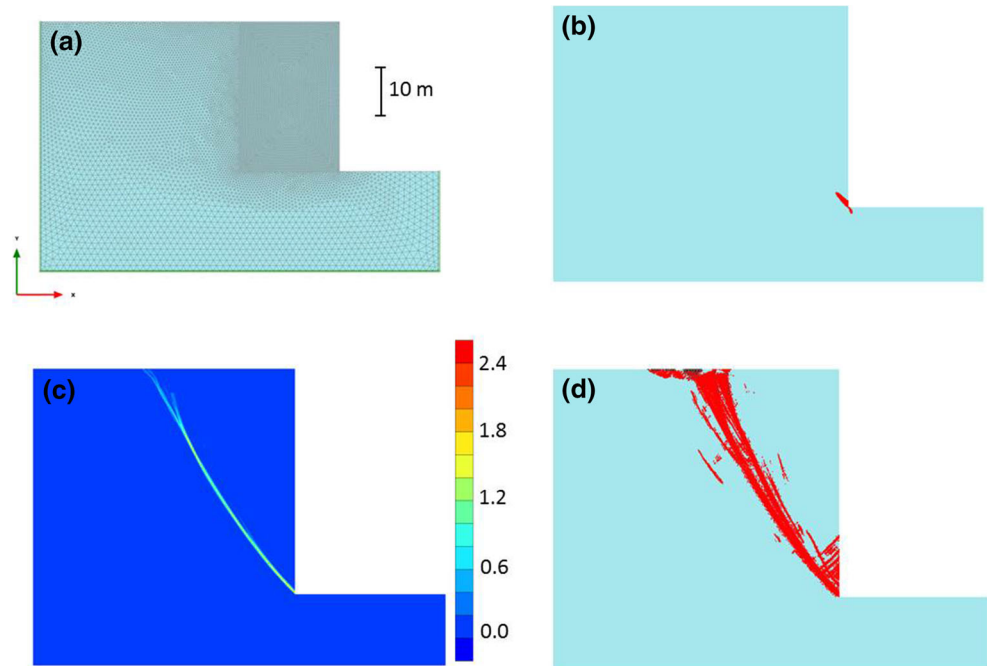
Fig. 19 FEM model of the vertical slope face: a discretization mesh; b plastic points ( red points ); c contours of deviatoric strains; and d plastic points ( red points ) and tensile failures ( black squares ) obtained from strength reduction analysis (colour figure online)
