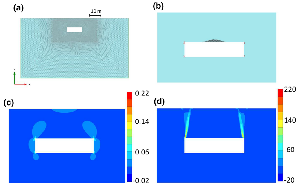
Fig. 16 FEM model of the 16 \times 4 m underground cavity: a discretization mesh; b plastic points ( red points ) and tensile failures ( black squares ); c contours of deviatoric strains; d contours of deviatoric strains obtained from strength reduction analysis (colour figure online)
