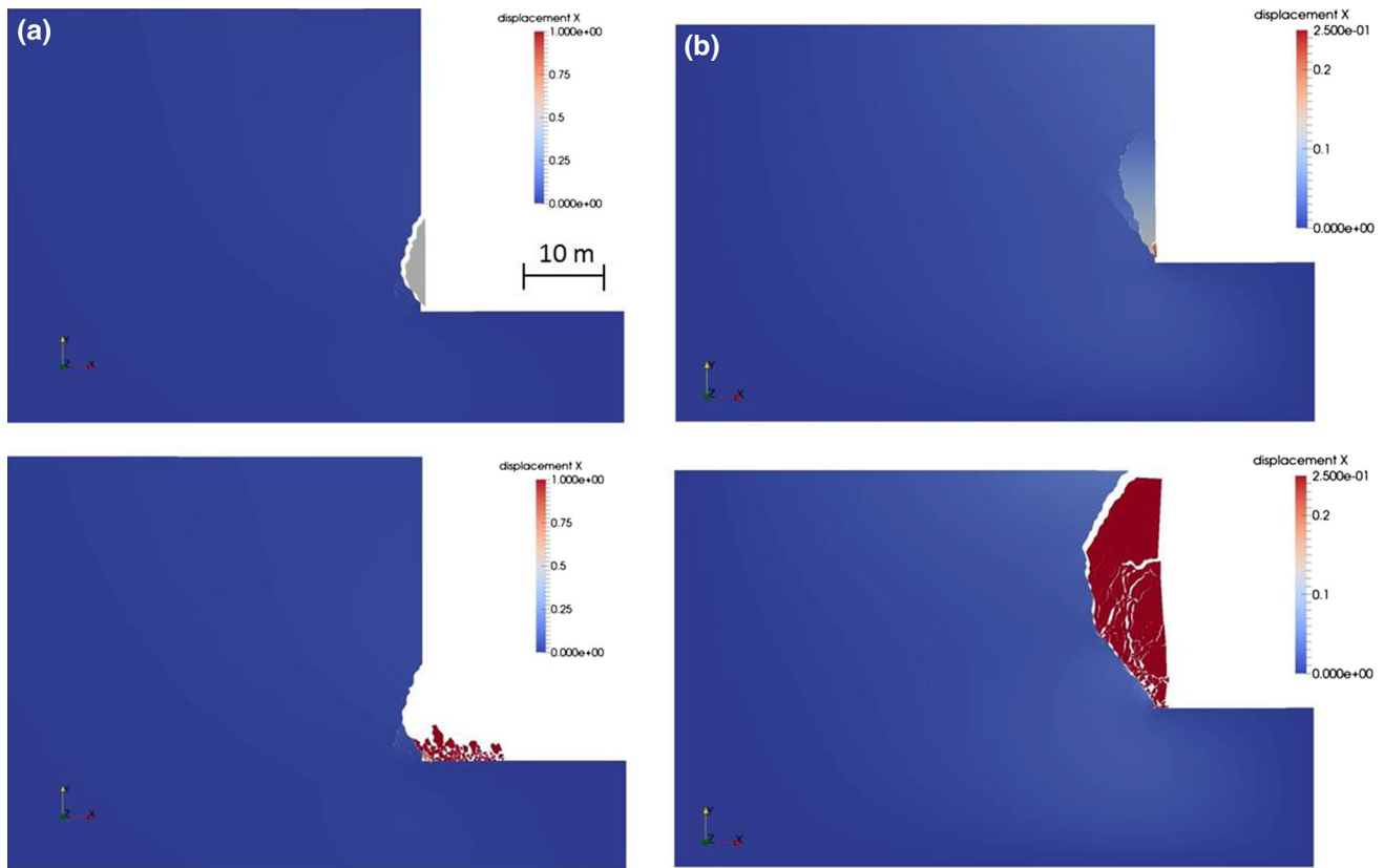
Fig. 21 Vertical slope face FDEM analysis: horizontal displacements obtained with a G_{If} = 20 N/m– G_{IIIf} = 200 N/m fracture energy parameters; b G_{If} = 10 N/m– G_{IIIf} = 100 N/m fracture energy parameters
