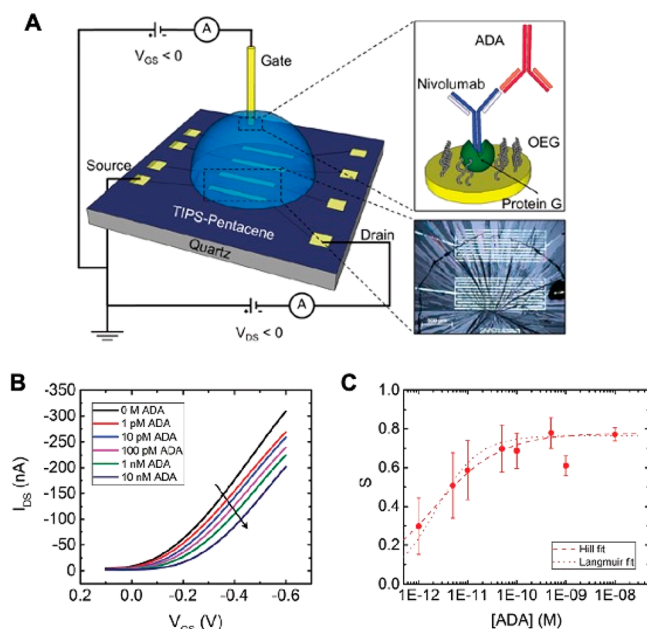
Figure 18. Schematic representation of the EG-FET device and the gate biofunctionalization protocol. (A) TIPS-pentacene is used as an organic semiconductor (in the inset is the optical microscopy picture). A PBS droplet is used as electrolyte. The zoomed-in view of the sensing gate is sketched in the of the inset. (B) Transfer characteristics registered after exposure to different concentrations of ADA, at V_{DS} = -0.2 V. (C) Semilog plot of the signal S as a function of the [\text{ADAs}] concentrations registered at V_{GS} = -0.2 V. Reprinted with permission from ref 97. Copyright 2021 The Royal Society of Chemistry under a Creative Commons Attribution-NonCommercial 3.0 Unported License.
