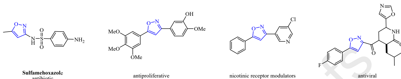
Figure 1. Some 3,5-disubstituted isoxazole based compounds with a spectrum of biological properties.
