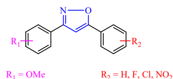
Figure 2. General structure of synthesized compounds.
