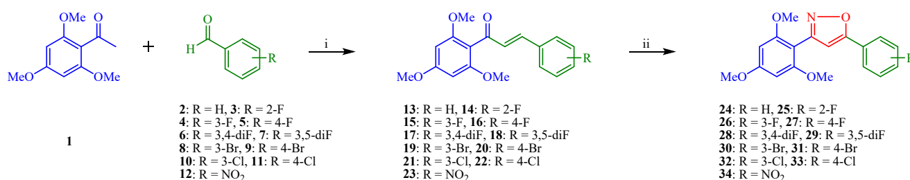
Scheme 1. General synthetic procedure. Reagents and conditions: (i) 1 , 2-12 , KOH, (ii) 13-23 , tosylhydroxylamine, K_2CO_3 , H_2O , MeOH
