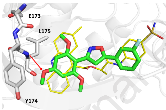
Figure 4. Zoomed in view at the binding pocket of S6K1 (PDB entry: 3WF9) whose residues are rendered in gray sticks and labeled. Green sticks and yellow wireframes represent 26 and F177 cognate ligand, respectively. Red arrows indicate hydrogen bonds.
