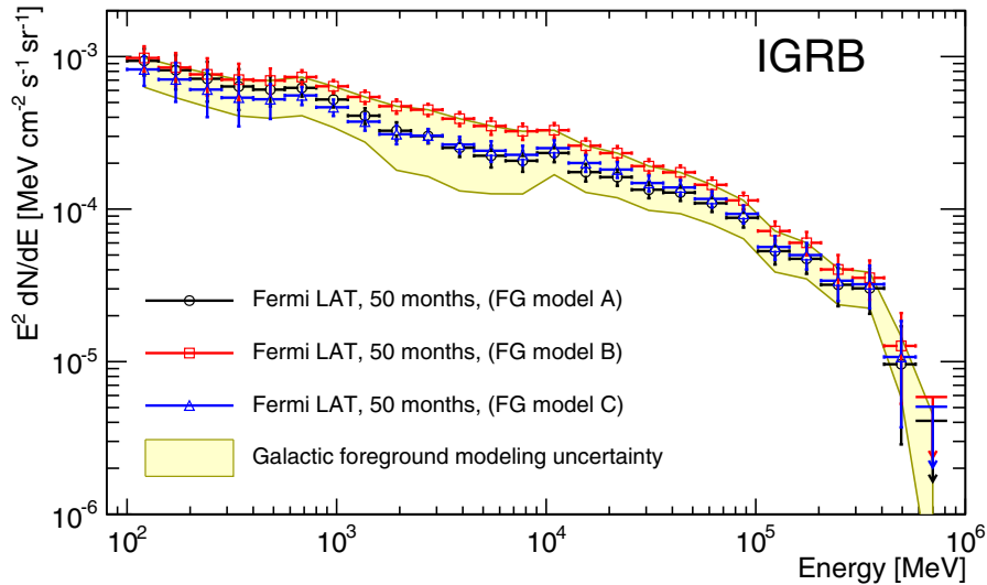
Figure 7. Comparison of the derived IGRB intensities for different foreground (FG) models. The error bars include the statistical uncertainty and systematic uncertainties from the effective area parameterization, as well as the CR background subtraction (statistical and systematic uncertainties have been added in quadrature). The shaded band indicates the systematic uncertainty arising from uncertainties in the Galactic foreground: the IGRB intensity range spanned by the three benchmark models, the variants described in Section 4.2, and the normalization uncertainties derived from the high-latitude data/model comparison. See Section 5.2 for details.
