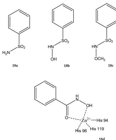
Figure 18. Compounds 18a–d [61].
