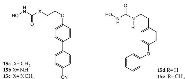
Figure 15. Compounds 15a–e [55].
