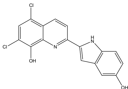
Figure 4. Compound WI-1758 [33].
