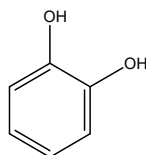
Figure 16. Catechol.
