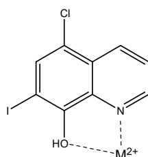
Figure 1. Clioquinol.
