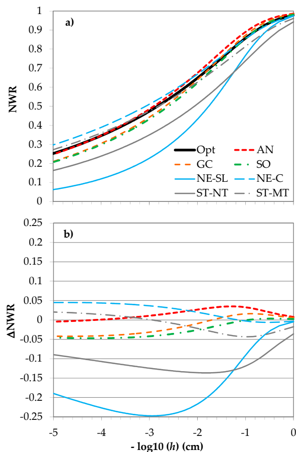
Figure 9. (a) Normalized water retention (NWR) of investigated soils plotted with the “optimal” (Opt) curve by Reynolds et al. [35], and (b) corresponding differences (estimated–optimal) in normalized water retention values ( \Delta\text{NWR} ) as a function of soil pressure head, h .
