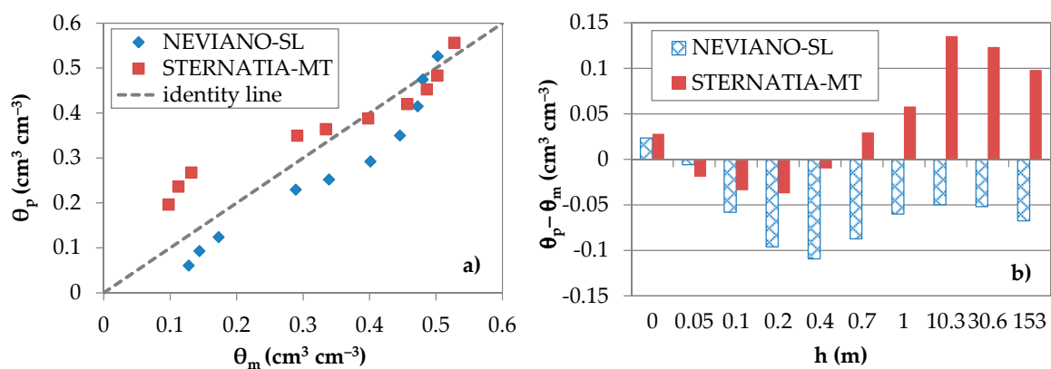
Figure 4. Comparison between predicted (θ p ) and measured (θ m ) soil water retention at Neviano and Sternatia sites (a) and corresponding differences as a function of soil pressure head (h) values (b).
