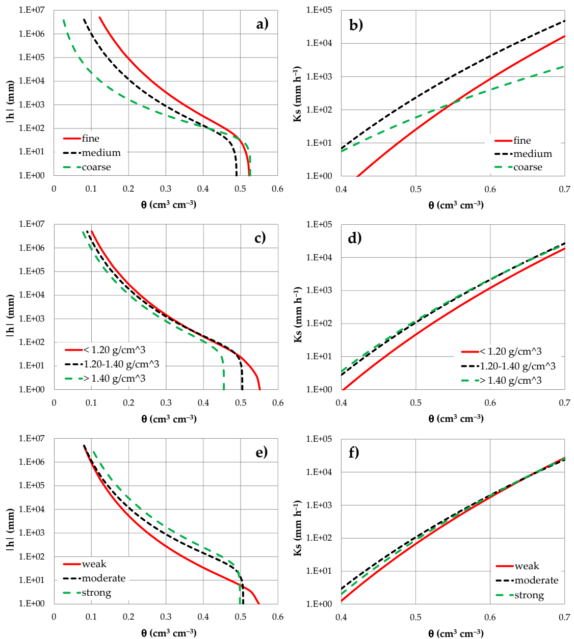
Figure 3. Soil water retention curve and hydraulic conductivity function (left and right, respectively) obtained for a given class of soil texture (fine, medium, and coarse; (a,b)), soil bulk density range (lower than 1.2 g cm -3 , between 1.2 and 1.4 g cm -3 , and higher than 1.4 g cm -3 ; (c,d)), or soil capillarity class (10 < λ c < 42 mm, 42 ≤ λ c ≤ 250 mm, and 250 ≤ λ c ≤ 1000 mm representing weak, moderate, and strong, respectively; (e,f)).
