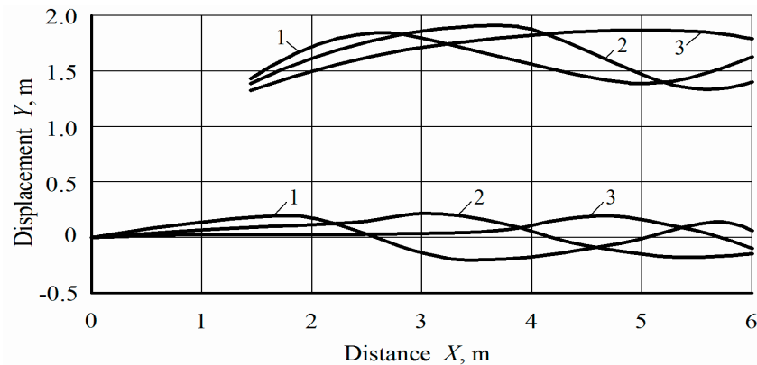
Figure 3. The trajectory of the motion of the center of mass of the root harvesting machine and the center of the outside digging working body at different velocities ( \text{m}\cdot\text{s}^{-1} ): 1 = 0.75; 2 = 1.68; 3 = 3.00.
