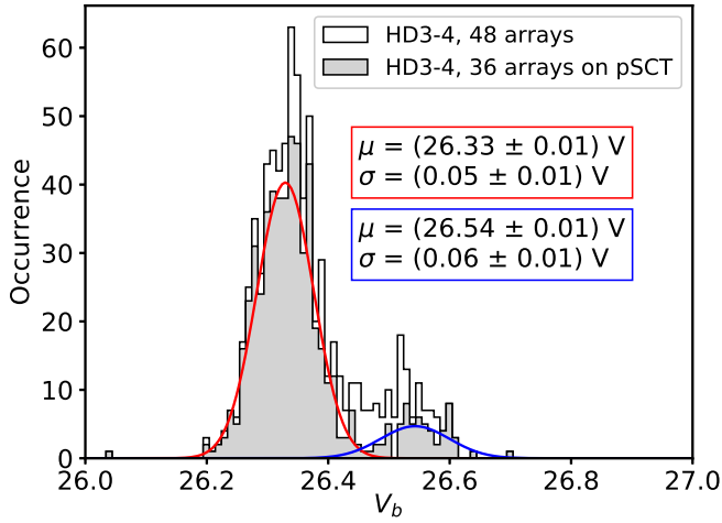
Figure 5: Distributions of the breakdown voltage for all the 48 SiPM arrays equipped with HD3-4 SiPMs (white) and for the 36 arrays installed on the pSCT camera (gray). The distribution of the arrays installed on the camera was fitted with two gaussian, one for each substrate of the SiPM production.
