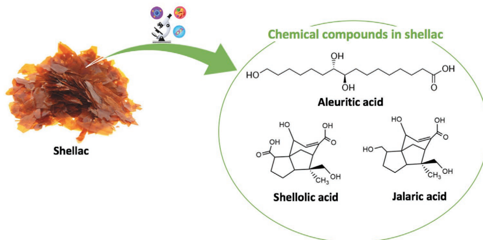
Figure 4. Main components of natural shellac.
