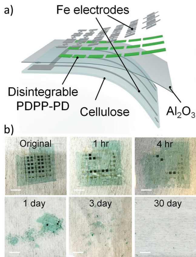
Figure 13. Totally disintegrable electronics fabricated with conventional deposition techniques. a) Schematic of the materials and device structure used for totally disintegrable electronics. The electrodes were deposited by thermal evaporation through a shadow mask, the \text{Al}_2\text{O}_3 insulating layer was deposited by atomic-layer-deposition and treated with SAM, and the PDPP-PD semiconductor was spin coated. b) Photographs of a device at various stages of disintegration. Scale bars: 5 mm. Reproduced with permission. [153] Copyright 2017, National Academy of Science.
