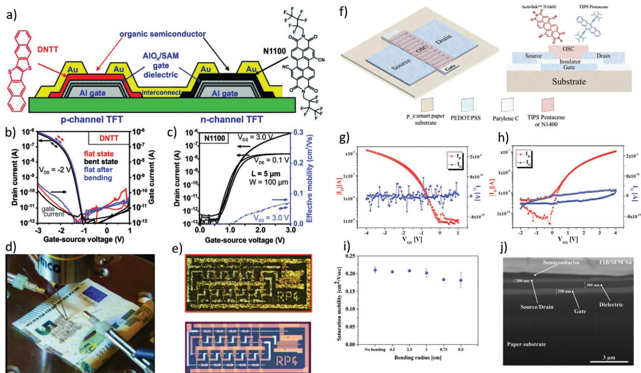
Figure 10. Organic transistors and circuits fabricated on paper substrates. a) Schematic cross-section of p-type (DNTT) and n-type (N1100) BG-TC OFETs connected in an inverter configuration. The Molecular structures of the organic semiconductors DNTT and Polyera ActivInk N1100 are showed. b) Transfer characteristics of a DNTT OFET on a banknote before, during and after bending. The channel length and width are 100 \mu\text{m} and the gate-to-contact overlap is 20 \mu\text{m} . Transfer characteristics of a N1100 OFET on a banknote. c) Transfer characteristics of a N1100 OFET fabricated on a banknote. d) Photograph of OFETs and circuits fabricated a banknote. e) Photographs of unipolar ring oscillators fabricated on a banknote (top) and on plastic PEN foil (bottom). Reproduced with permission from. [148] Copyright 2018, Wiley-VCH. f) Schematic 3D view and cross-section of BG-BC printed OFETs on commercial paper substrate. g) Transfer characteristic and gate leakage current of a p-type TIPS pentacene OFET. h) Transfer characteristic gate leakage current of a n-type ActivInk N1400 OFET. i) Average saturation mobility of p-OFETs before and during bending at different radius ( R = 45, 25, 10, 7.5, and 5 \text{ mm} ). Error bars are the standard deviation. j) FIB-SEM image of an OFET cross-section. The various materials are highlighted. Reproduced with permission. [158] Copyright 2020, Wiley-VCH.
