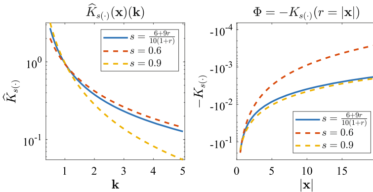
Fig. 1 Plots of \widehat{K}_{s(\cdot)}(x)(k) and \Phi = -K_{s(\cdot)}(r = |\mathbf{x}|)
