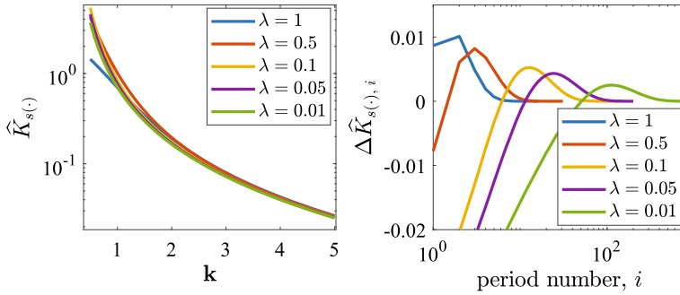
Fig. 2 Plots of \widehat{K}_{s(\cdot)} for different values of \lambda vs the frequency k (left) and \Delta \widehat{K}_{s(\cdot), i} for k = 5 for different values of \lambda vs the period number i (right). As expected the convergence is slower for small \lambda . The positive local maximum for \Delta \widehat{K}_{s(\cdot), i} occurs around i \approx ak\lambda^{-1}
