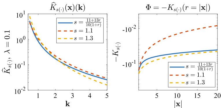
Fig. 4 Plots of \widehat{K}_{s(\cdot)}(\mathbf{x})(\mathbf{k}) and \Phi = -K_{s(\cdot)}(r = |\mathbf{x}|)
