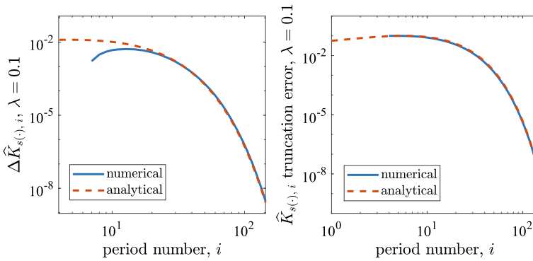
Fig. 3 Plots of \Delta \widehat{K}_{s(\cdot), i} computed numerically and with Eq. (4.3) (left) and the truncation error estimated numerically and with Eq. (4.4) (right) for k = 5
