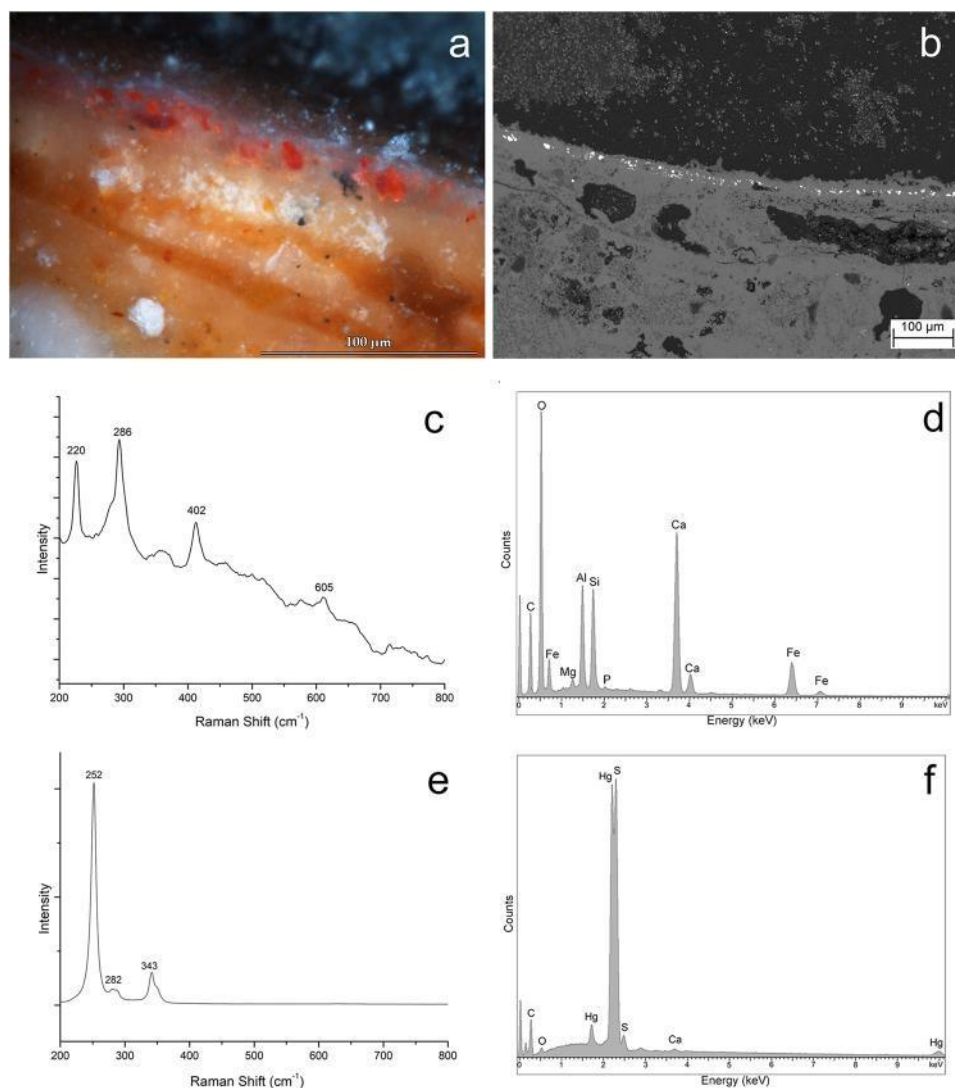
Fig. 4 Microphotograph showing the red layers in the sample CR5 (first cycle of the Christ Pantocrator painting), namely the orange-red ochre (colour R3) layers and on the top the layer of cinnabar (colour R4) (a); BSE-SEM image of the same sample, showing, on the surface, the cinnabar (HgS) pigment particle, which appear very lucent (b); micro-Raman spectrum of red ochre (c) ( \lambda_0 = 638 nm, 5 mW, 1-s exposure time, 20 accumulations) and cinnabar (e), both identified in the CR5 sample ( \lambda_0 = 638 nm, 5 mW, 1-s exposure time, 20 accumulations); SEM-EDS spectra of red ochre (d) and cinnabar (f), showing their typical compositions
