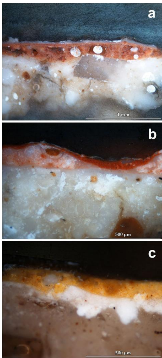
Fig. 9 Microphotographs showing the absence of the plaster layer in the Christ Pantocrator (a) and Virgin with Child (b) paintings and the presence of a white, thin and not continuous layer in the St. Michael painting (c), probably correlated to the presence of intonaco
