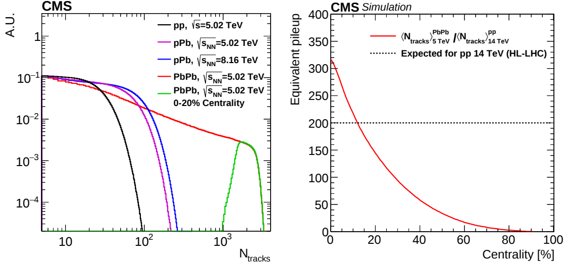
Figure 2. Left: Distribution of N_{\text{tracks}} in pp collisions at \sqrt{s} = 5.02 TeV (black); pPb collisions at \sqrt{s_{NN}} = 5.02 TeV (magenta) and at \sqrt{s_{NN}} = 8.16 TeV (blue); and PbPb collisions at \sqrt{s_{NN}} = 5.02 TeV (red). The distribution of N_{\text{tracks}} in the 0–20% most central PbPb collisions is shown in green. The values are not corrected for efficiency. Right: Translation of the centrality in PbPb collisions at \sqrt{s_{NN}} = 5.02 TeV into an equivalent pileup in pp collisions at \sqrt{s} = 14 TeV.
