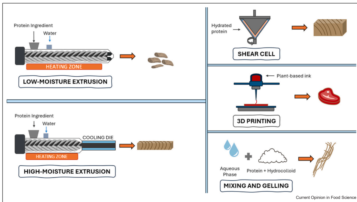
Texturization technologies for the development of meat analogs and materials with fibrous texture.
