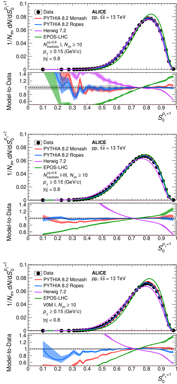
Figure 1. Upper panels: the measured and fully corrected S_0^{p_T=1} distributions. Lower panels: ratio between model calculations and experimental data. These are presented for N_{tracklets}^{|\eta| < 0.8} I (top), I–III (middle) and V0M I (bottom). The roman numerals I (I–III) correspond the top 0–1% (0–10%) multiplicity for each respective estimator. The curves represent different model predictions, where the shaded area represents the statistical uncertainty of the models. The relative systematic uncertainty is shown as a gray area around unity in the lower panels.
