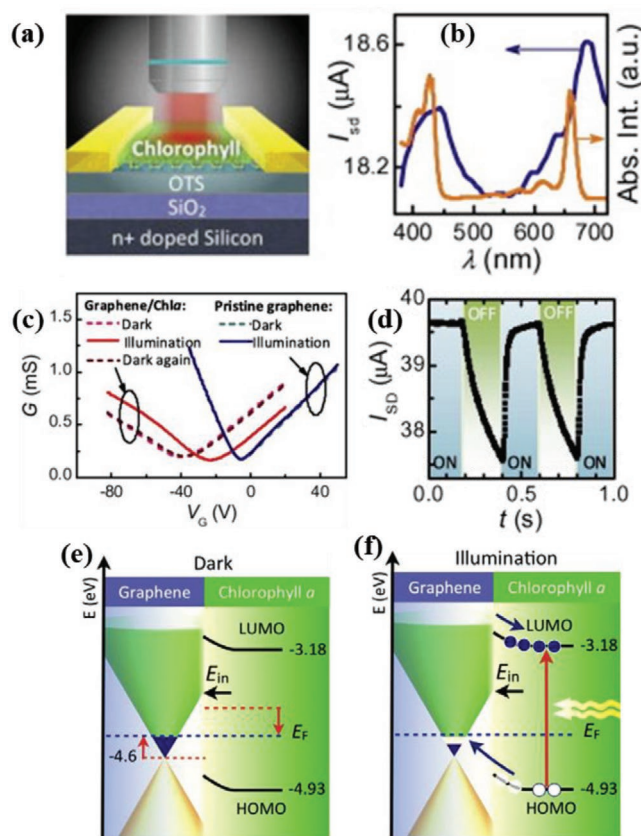
Figure 12. a) Scheme of the graphene-Chl device. b) Photocurrent action spectrum of graphene-Chl (blue line) overlap with the absorption spectrum of Chl (orange line). c) G-V_G curves of pristine graphene and graphene-Chl with and without illumination (683 nm). d) Photocurrent dynamics of graphene-Chl upon cycles of dark and light (200 ms each). Diagram of the energy level of e) n-doping effect graphene-Chl when the light is off and f) relative variation upon illumination. Reproduced with permission. [31] Copyright 2013, Elsevier Ltd.
