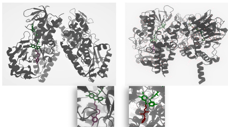
Fig. 1. Crystal structures of hMAO isoforms taken from PDB [16]. Left side: complex of hMAO A with clorgyline (PDB 2BXR). Right side: complex of hMAO B with selegiline (PDB 2BYB). For both complexes, magnifications evidence the inhibitors (red) covalently bound to cofactor FAD (green).
