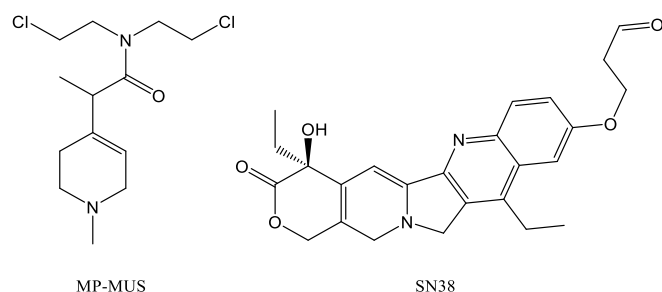
Fig. 7. Chemical structures of MP-MUS and SN38.
