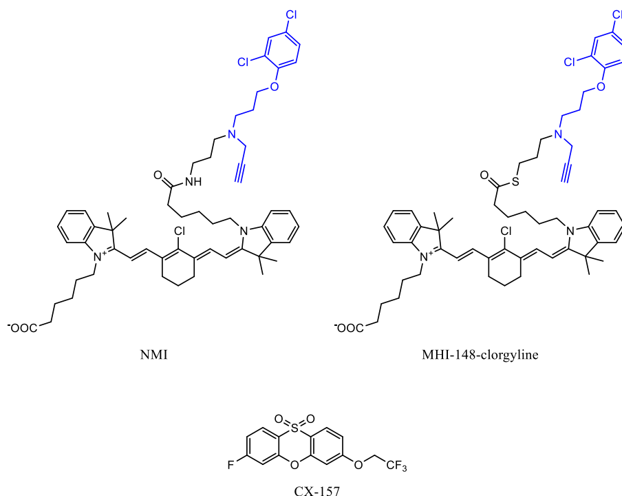
Fig. 6. Chemical structures of the clorgyline derivatives NMI and MHI-148-clorgyline and CX-157.
