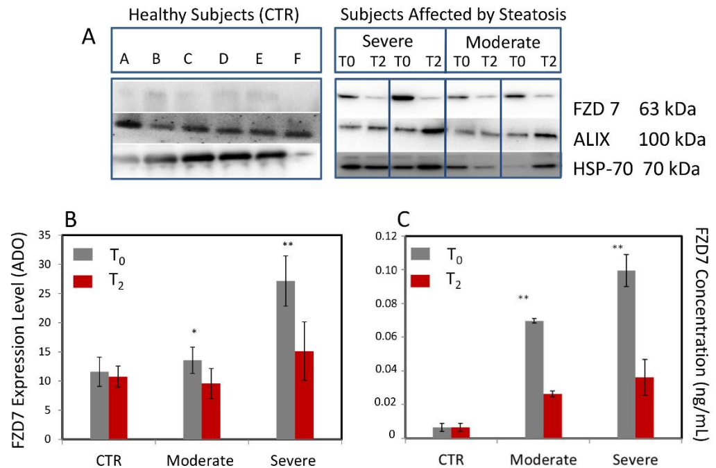
Figure 2. Exosomes extracted from plasma of all healthy subjects (20) and NAFLD-affected patients (95) with moderate (38) or severe (57) hepatic steatosis at recruitment time (T0) and after treatment (T2): (A) representative Western Blotting of FZD7, ALIX, and HSP-70 (molecular mass markers are indicated on the right); (B) semi-quantitative estimation, by Western blotting analysis and densitometry of protein bands, of relative FZD7 expression level; (C) quantitative analysis of FZD7 by ELISA assay. For semiquantitative analysis, the same total protein content (20 \mu g) was loaded and FZD7 bands were evaluated upon normalization with the corresponding housekeeping ALIX protein band for each sample. * p < 0.05 and ** p < 0.001 versus control.
