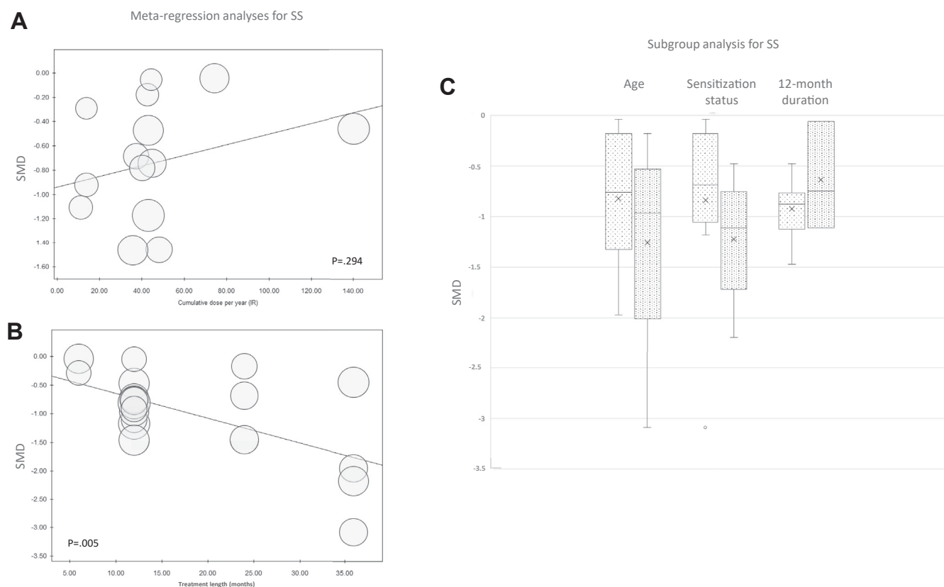
FIG 3. Metaregression analyses of SS for efficacy of IR-HDM SLIT liquid depending on cumulative dose administered per year ( A ) or treatment length ( B ). ( C ) Subgroup analysis box plots include middle 50% of data. Horizontal bars inside boxes represent SMD; lines to whiskers extend most extreme data points, which are no more than 1.5 times interquartile range from box.
