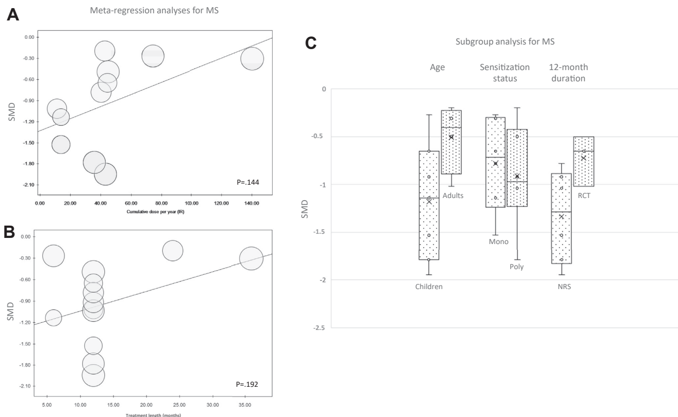
FIG 5. Metaregression analyses of MS for efficacy of IR-HDM SLIT liquid depending on cumulative dose administered per year ( A ) or treatment length ( B ). ( C ) Subgroup analysis box plots include middle 50% of data. Horizontal bars inside boxes represent SMD; lines to whiskers extend most extreme data points, which are no more than 1.5 times interquartile range from box.
