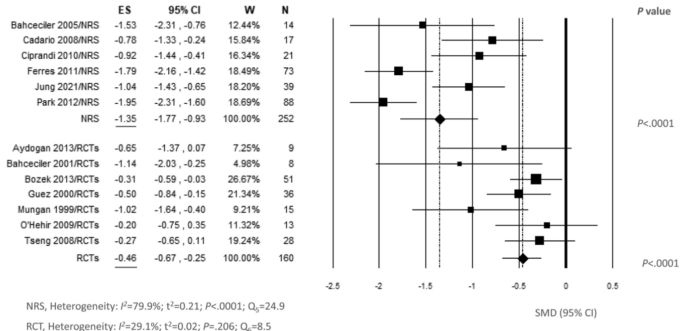
FIG 4. Meta-analysis of 6 NRS and 7 RCT of IR-HDM SLIT liquid baseline versus end of treatment for ARC using random effects model (REM). SMD and 95% CI for effect of SLIT on MS are plotted on graph. Studies of each group are arranged in alphabetic order. ES, Estimate; W, weights.
