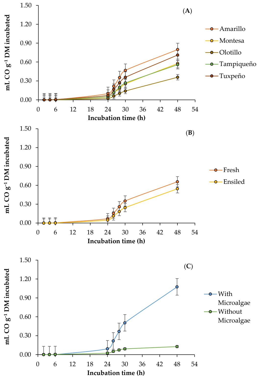
Figure 3. Kinetics of ruminal carbon monoxide (CO) production from maize forage in response to genotype: (A) Amarillo, Montesa, Olotillo, Tampiqueño, and Tuxpeño states of forage; (B) fresh or ensiled; (C), with or without D. salina .
