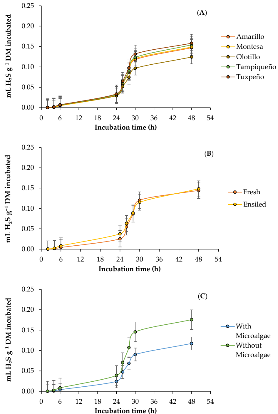
Figure 4. Kinetics of ruminal hydrogen sulfide ( \text{H}_2\text{S} ) production from maize forage in response to genotype: (A) Amarillo, Montesa, Olotillo, Tampiqueño, and Tuxpeño states of forage; (B) fresh or ensiled; (C) with or without D. salina .
