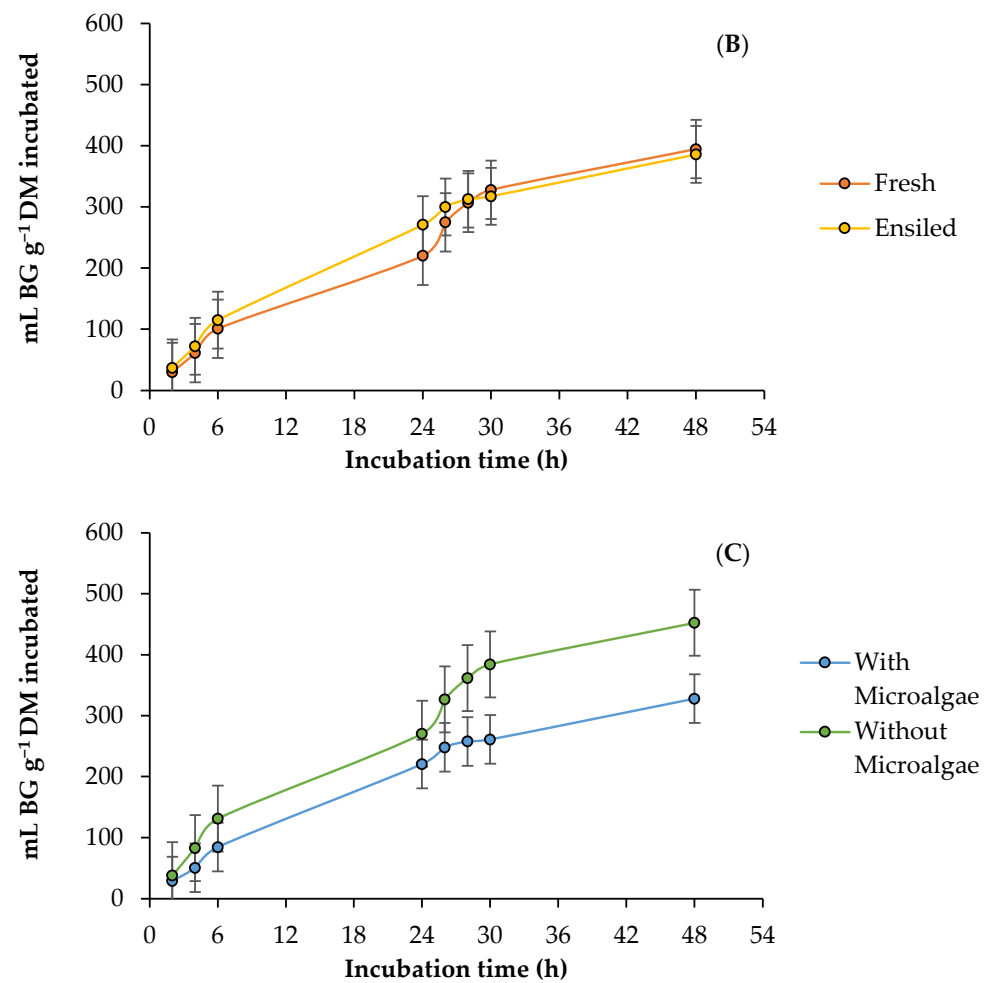
Figure 1. Kinetics of ruminal biogas (BG) production from maize forage in response to genotype: (A) Amarillo, Montesa, Olotillo, Tampiqueño, and Tuxpeño states of forage; (B) fresh or ensiled; (C) with or without D. salina .
