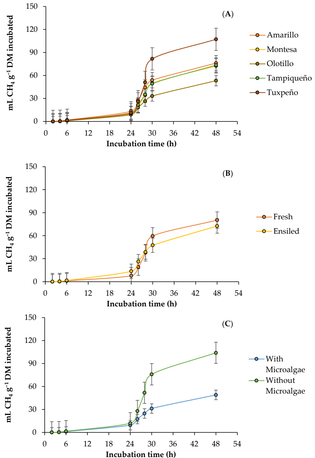
Figure 2. Kinetics of ruminal methane ( \text{CH}_4 ) production from maize forage in response to genotype: (A) Amarillo, Montesa, Olotillo, Tampiqueño, and Tuxpeño states of forage; (B) fresh or ensiled; (C) with or without D. salina .
