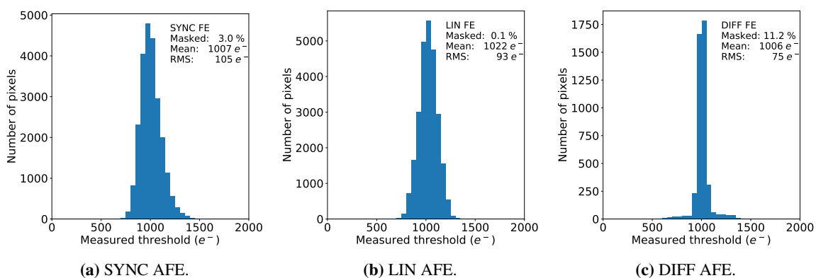
Figure 14. Threshold distributions of the SYNC AFE (a), the LIN AFE (b), and the DIFF AFE (c) obtained with an RD53A chip after irradiation. The mean and RMS were calculated using all non-masked pixels in each AFE.
