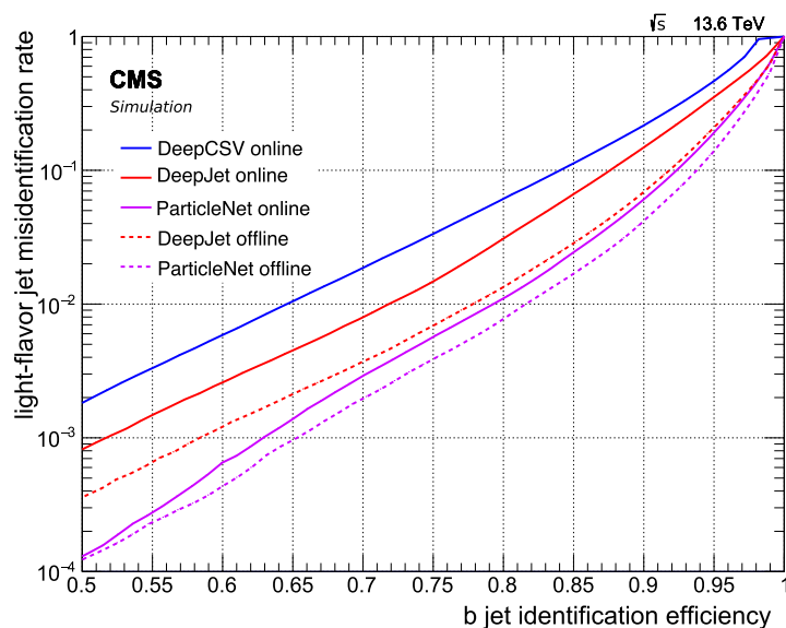
Figure 132. Light-flavor jet misidentification rate versus the b jet efficiency for the various b tagging algorithms. The solid curves show the performance of the DeepCSV (blue), DeepJet (red), and ParticleNet (magenta) algorithms in the HLT. The dashed curves show the corresponding offline performance for DeepJet (red) and ParticleNet (magenta) taggers using offline reconstruction and training.
