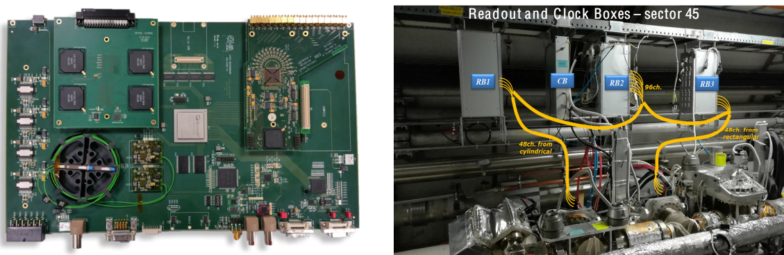
Figure 101. Left: the digital readout unit. In this example both an HPTDC mezzanine (upper left) and a SAMPIC mezzanine (upper right) are mounted on the motherboard. Right: location of PPS mini-crates installed above the LHC beam pipe, for both the cylindrical timing RP already used in Run 2, and the rectangular 220-N RP newly equipped for timing in Run 3. The readout boxes (labeled “RB”) contain the NINO boards and DRUs as described in the text. The box labeled “CB” holds components for the precise reference clock.
