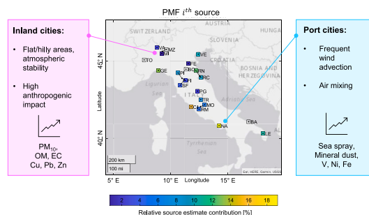
PM 10 chemical speciated data from 21 Italian cities (years 2005–2016)
