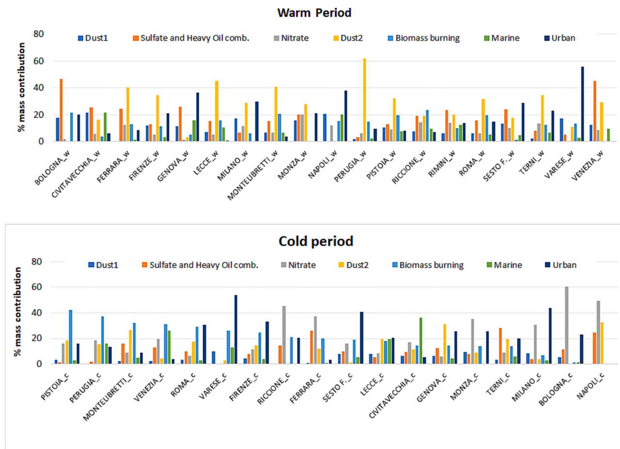
Fig. 6. Mean PM 10 source contributions (in %) averaged over all results retrieved for the warm (w) and cold (c) periods at each investigated site.
