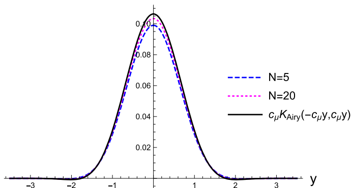
Fig. 5 The kernel at the edge K_{N, \sqrt{2\mu}, \hbar^{\frac{2}{3}}}^2(-y, y) compared to its limit c_{\mu} K_{Ai}(-c_{\mu}y, c_{\mu}y) . Here \mu = 2 . Note the integrable tails (see Lemma 4)
