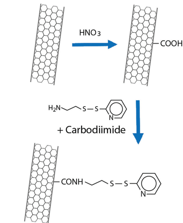
Figure 5. Synthetic pathway for the thiolation of carbon nanotubes. [80]
