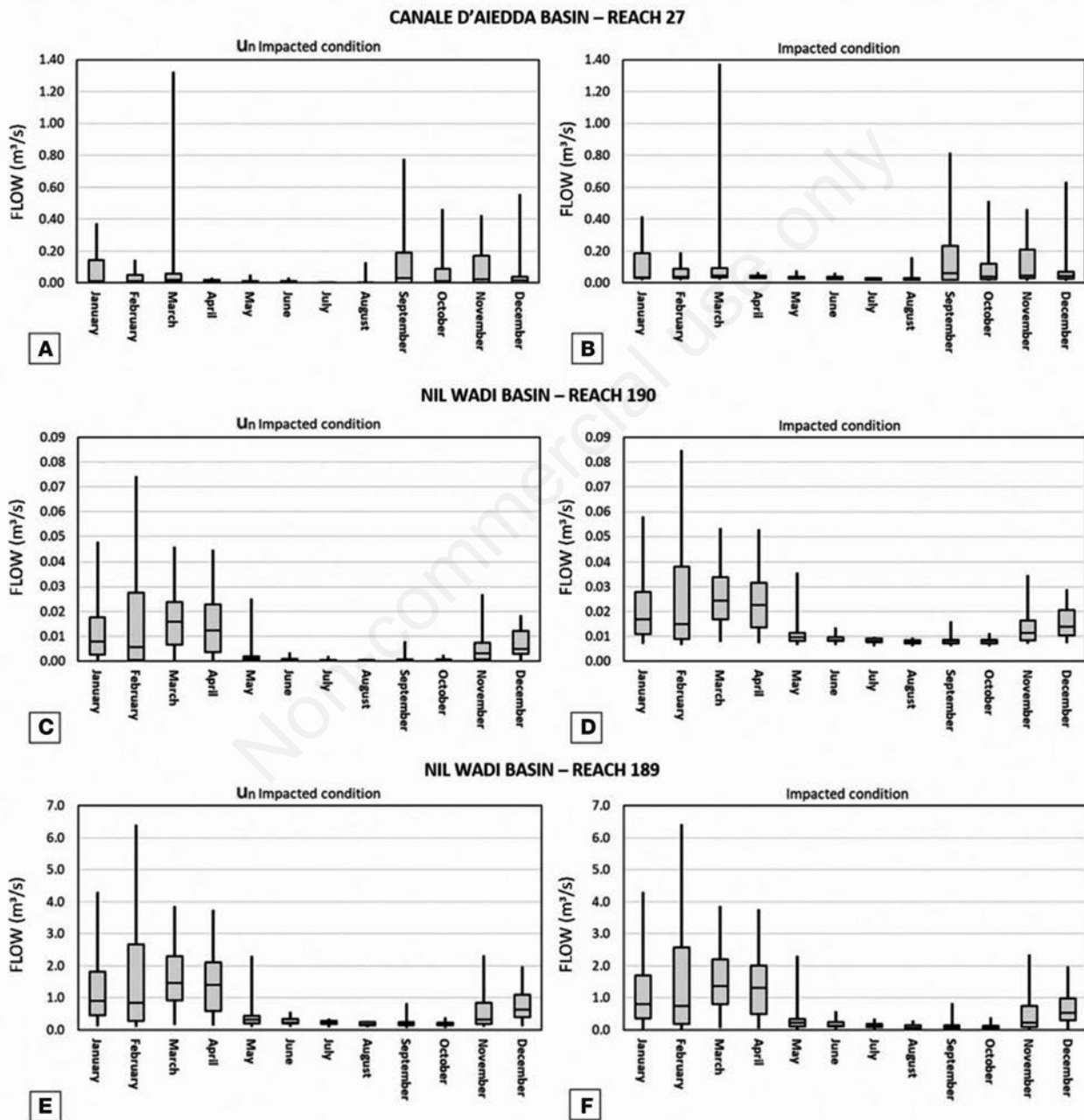
Figure 6. Box plot of monthly flow ( \text{m}^3\text{s}^{-1} ) in un-impacted and impacted conditions. The horizontal line within the boxplots indicates the median value, the box boundaries indicate the 25 th and 75 th percentiles, and the whiskers indicate the minimum and 95 th percentile.
