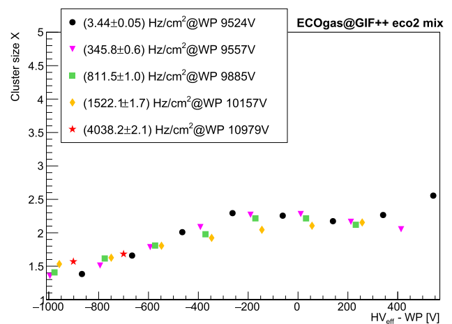
Fig. 11 Average muon cluster size as a function of the relative difference between the HV_{eff} and the detector WP for the eco2 gas mixture. Results are shown for the vertical strip plane, at 6m (top) and 3m (bottom) from the source and at different gamma cluster rates (efficiency corrected) evaluated at the detector WP
