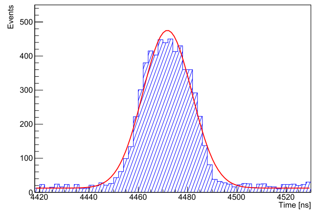
Fig. 3 Typical muon window as defined in the 5 \mu s trigger time interval
