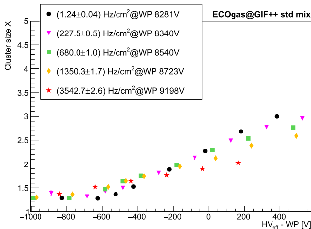
Fig. 10 Average muon cluster size as a function of the relative difference between the HV_{eff} and the detector WP for the standard gas mixture. Results are shown for the vertical strip plane, at 6m (top) and 3m (bottom) from the source and at different gamma cluster rates (efficiency corrected) evaluated at the detector WP
