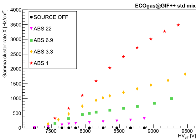
Fig. 4 Gamma cluster rate as a function of HV_{\text{eff}} for the thin-RPC operated with standard gas mixture. Results are shown for the vertical strip plane, at 6 m (top) and 3 m (bottom) from the source
