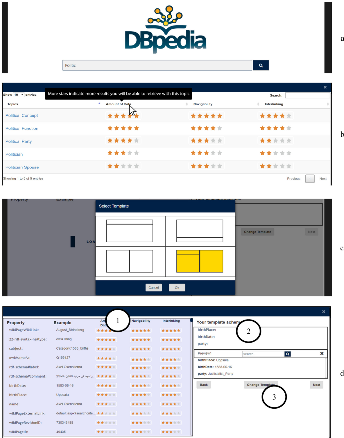
Fig. 1. MDS creation process. The users have to: (a) type one or more keywords to indicate the topics they are interested in; (b) select a topic from the list of topics semantically related to the user keyword; (c) choose a UI template to visualize the MDS results; (d) map topic properties into the chosen template.
