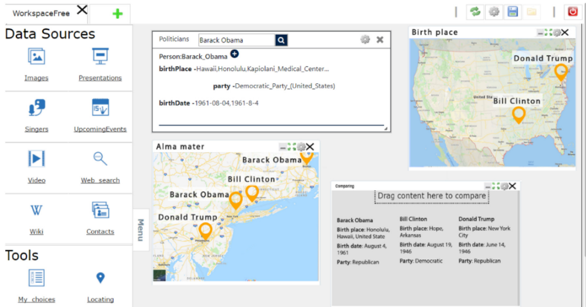
Fig. 4. Example of an interactive workspace with an MDS that retrieve US Presidents and three tools (two Maps and one Comparing component) to manipulate and visualize the MDS results.
