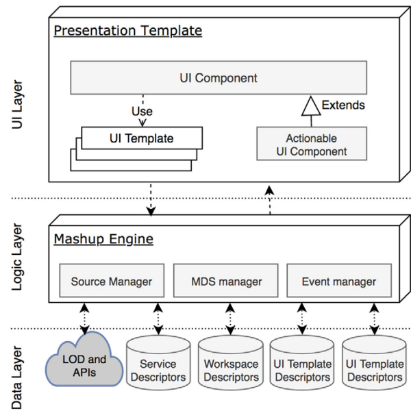
Fig. 6. A high-level overview of the EFESTO three-layer architecture.
