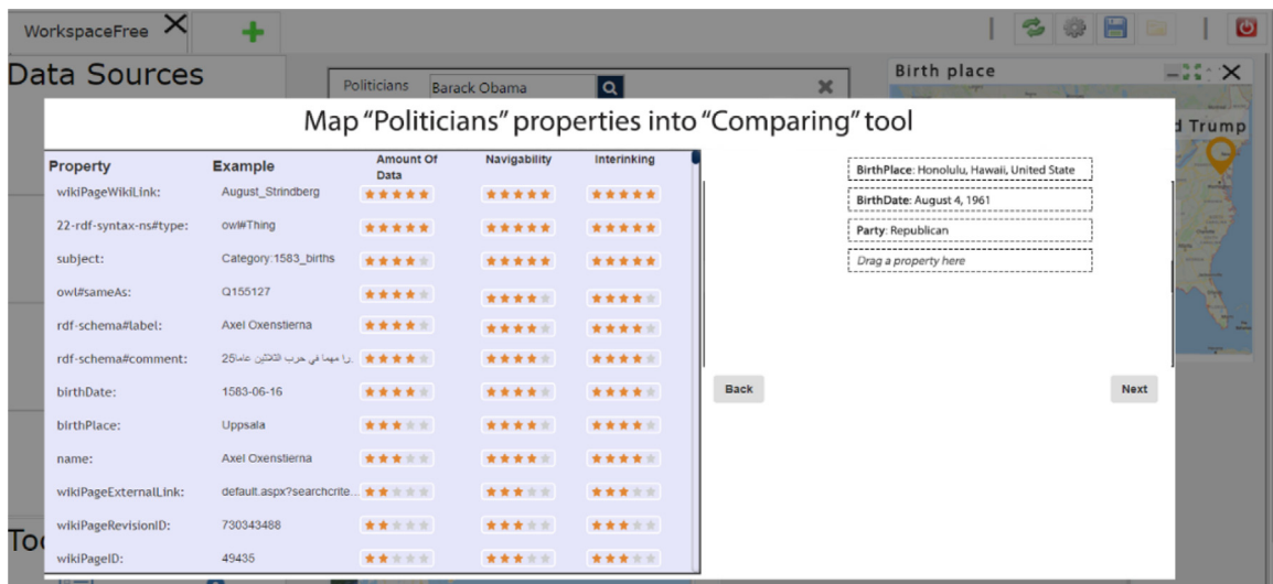
Fig. 5. Training by the user of an Actionable UI Component (Comparing tool in the example): drag&drop actions map three MDS class properties (Politicians properties) onto the capability of the Actionable UI Component (textual fields displaying the attributes to compare).
