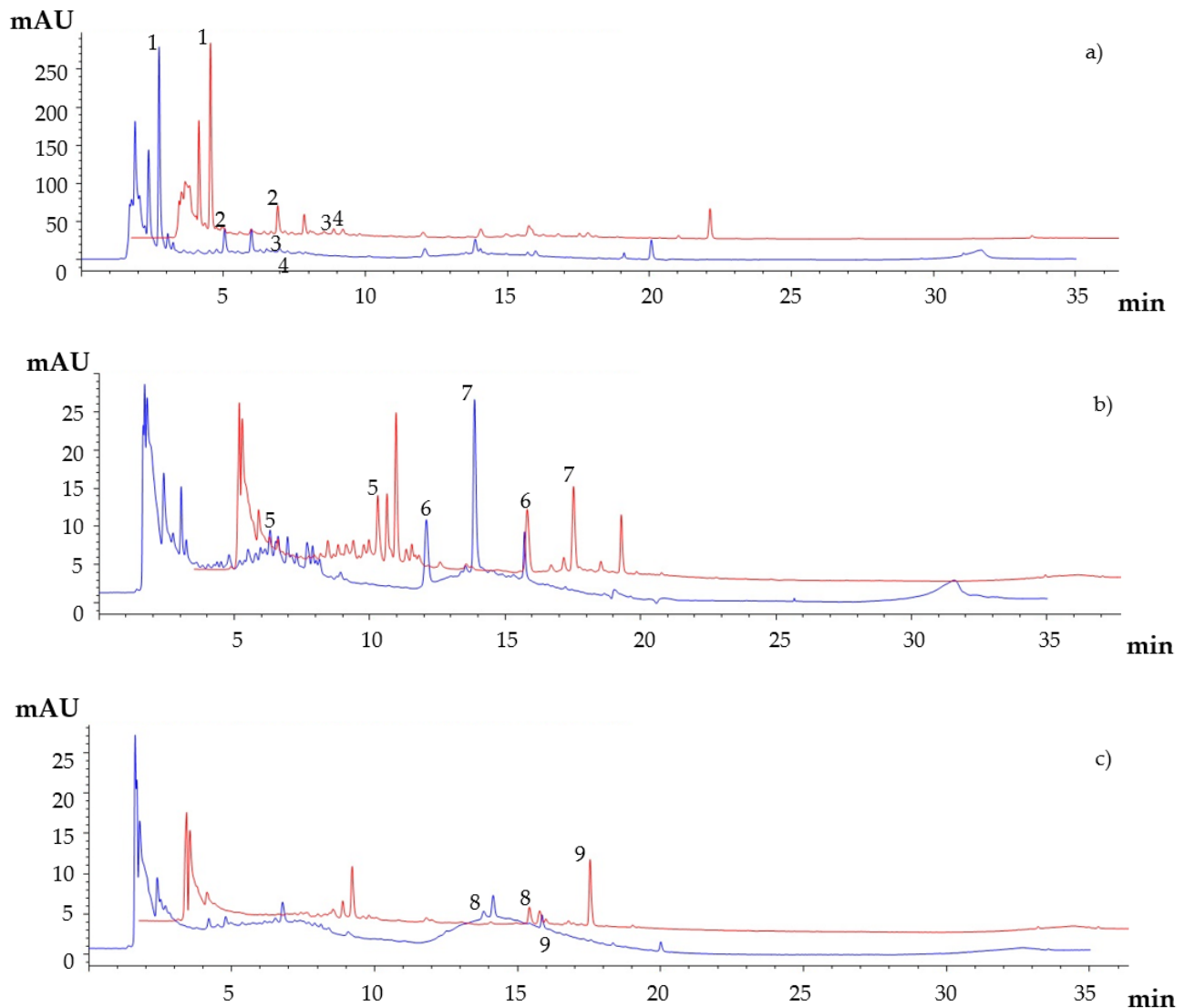
Figure 5. HPLC-DAD chromatograms at (a) 280 nm, (b) 330 nm, (c) 360 nm of traditional (blue line) and UAE (red line) carob syrup diluted 1:3. 1: gallic acid (2.733 min), 2: procyanidin B 1 (5.001 min), 3: procyanidin B 2 (7.091 min), 4: epicatechin (7.879 min), 5: chlorogenic acid (6.229 min), 6: 4-hydroxycoumaric acid (12.205 min), 7: ferulic acid (13.939 min), 8: myricitrin (13.531 min), 9: quercitrin (15.701 min).
