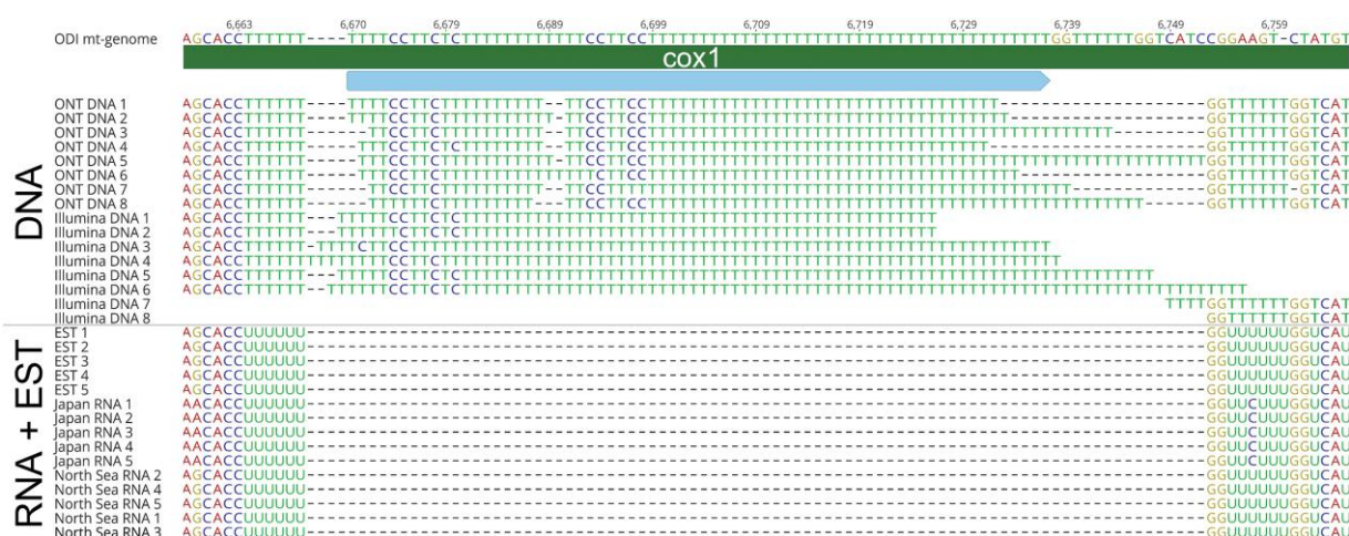
Fig. 2. A typical poly-A/T region in the O. doica cox1 gene. The reference sequence represents the assembled mitochondrial genome. The sequence of part of the cox1 gene is indicated in dark green. Above it are the nucleotide and amino acid sequences of the reference sequence. The poly-A/T region is in light blue. Reads from five different sequencing sources mapped to this region are shown below the reference sequence: our ONT data, our Illumina reads, public EST data from Norway, public RNA reads from Japan, and public RNA reads from the North Sea (see supplementary table S3a, Supplementary Material online for accession numbers). Each line represents a different read. Note that the different ONT reads do not have the same length, exemplifying the fact that the length of the poly-T region could not be accurately determined. The EST and RNA reads lack a long poly-U region. Rather, the poly-T region corresponds to 6U-bases. This difference (long poly-T stretch in DNA vs. 6U in the EST and RNA reads) provides evidence of editing at the RNA level. Illumina reads can map to each side of the poly-T stretch, but because poly-T stretches can be longer than the read length, we were unable to assemble the entire region using Illumina only or to determine the length of the poly-T region.
