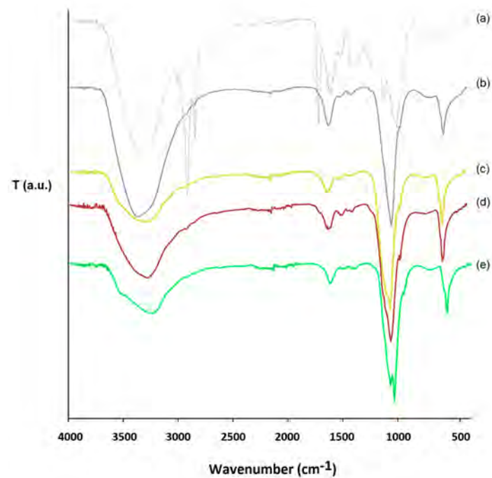
Figure 7. ATR spectra of (a) dried cells after recovery from culture medium (fresh diatoms) and after purification with acid-oxidative protocol of (b) bare, (c) Ir-doped, (d) Ru-doped, and (e) Al-doped shells.
