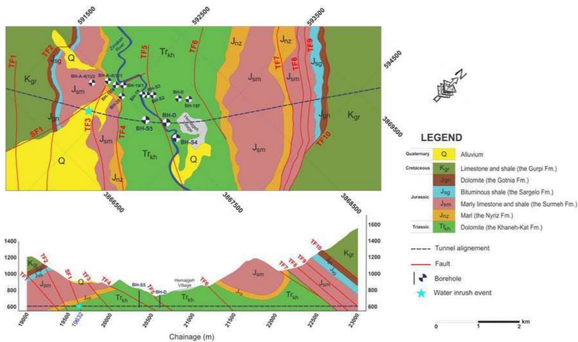
Fig. 3 Geological map and profile of the Nosud Tunnel in the Zimakan Valley (chainage 19 to 23 km)
