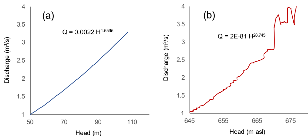
Fig. 1 Head-discharge relationship for a 1.2-m Parshall Flume device and b the Nosud Tunnel
