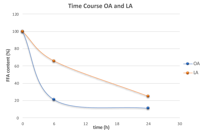
Fig. 2. Time course of oleic acid (OA, blue) and linoleic acid (LA, orange) consumption by the enzyme Em_OhyA starting from WCO-derived FFA.
