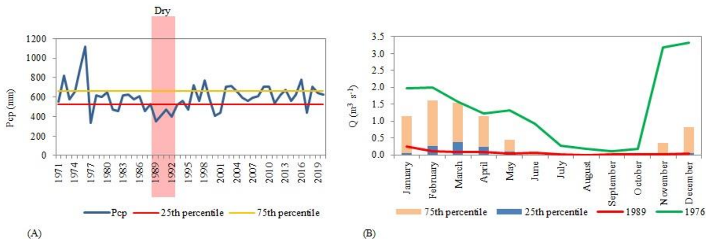
Fig. 5. Annual rainfall amount at the basin scale, 25 th percentile and 75 th percentile over the period 1971 to 2020 (A). The magnitude of monthly flow for a dry year (1989) and wet year (1976) and 25 th and 75 th percentiles computed over the period 1971 to 2020 (B).
