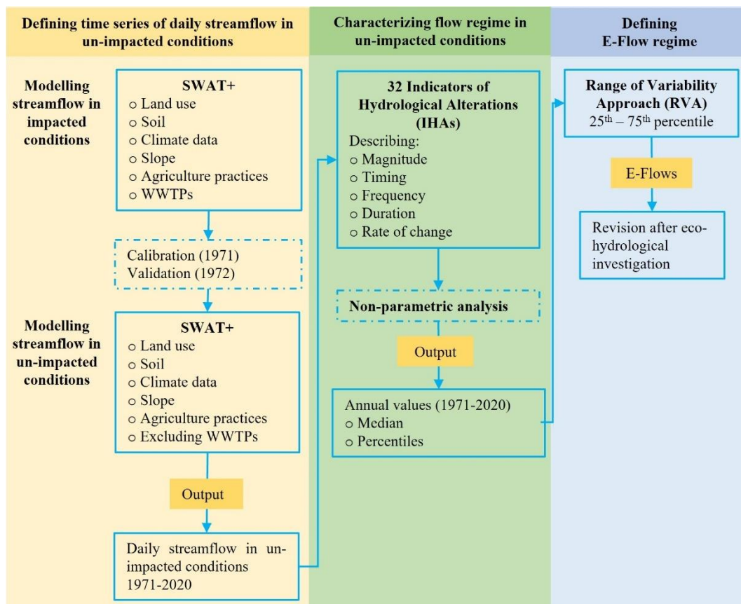
Fig. 2. Schematic overview of the methodology. IHAs were calculated from 1971 to 2020. E-Flow regime was set fixing each IHA within the inter-quartile range of its natural variability.
