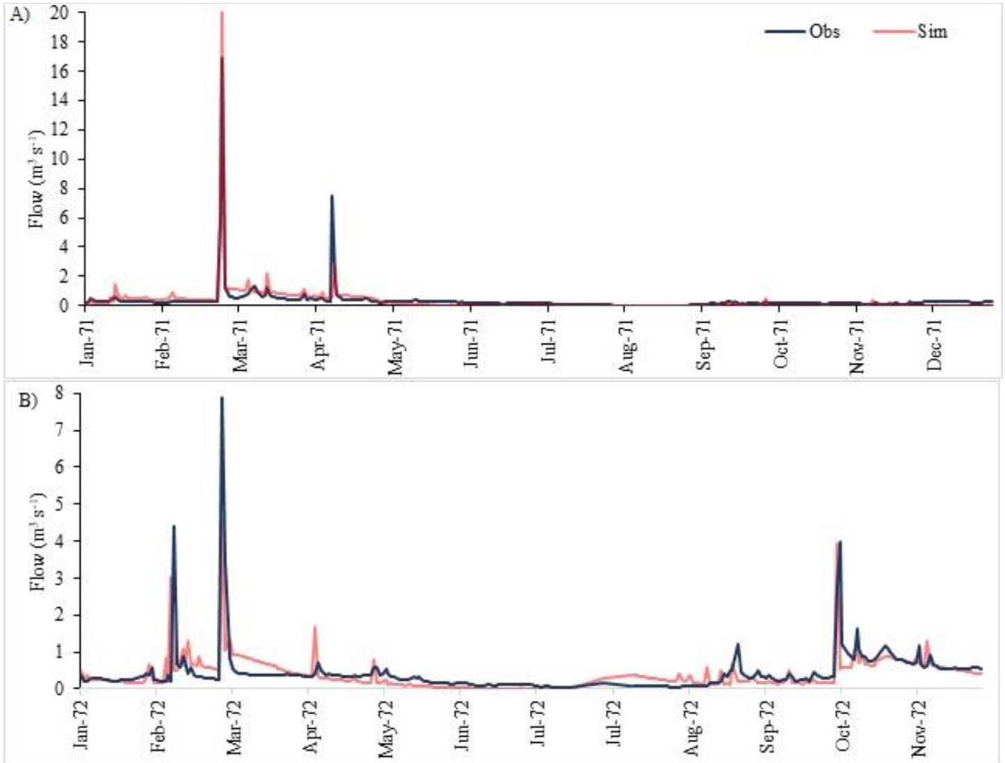
Fig. 3. Observed and simulated daily streamflow. A) Calibration (1971). B) Validation (1972).
