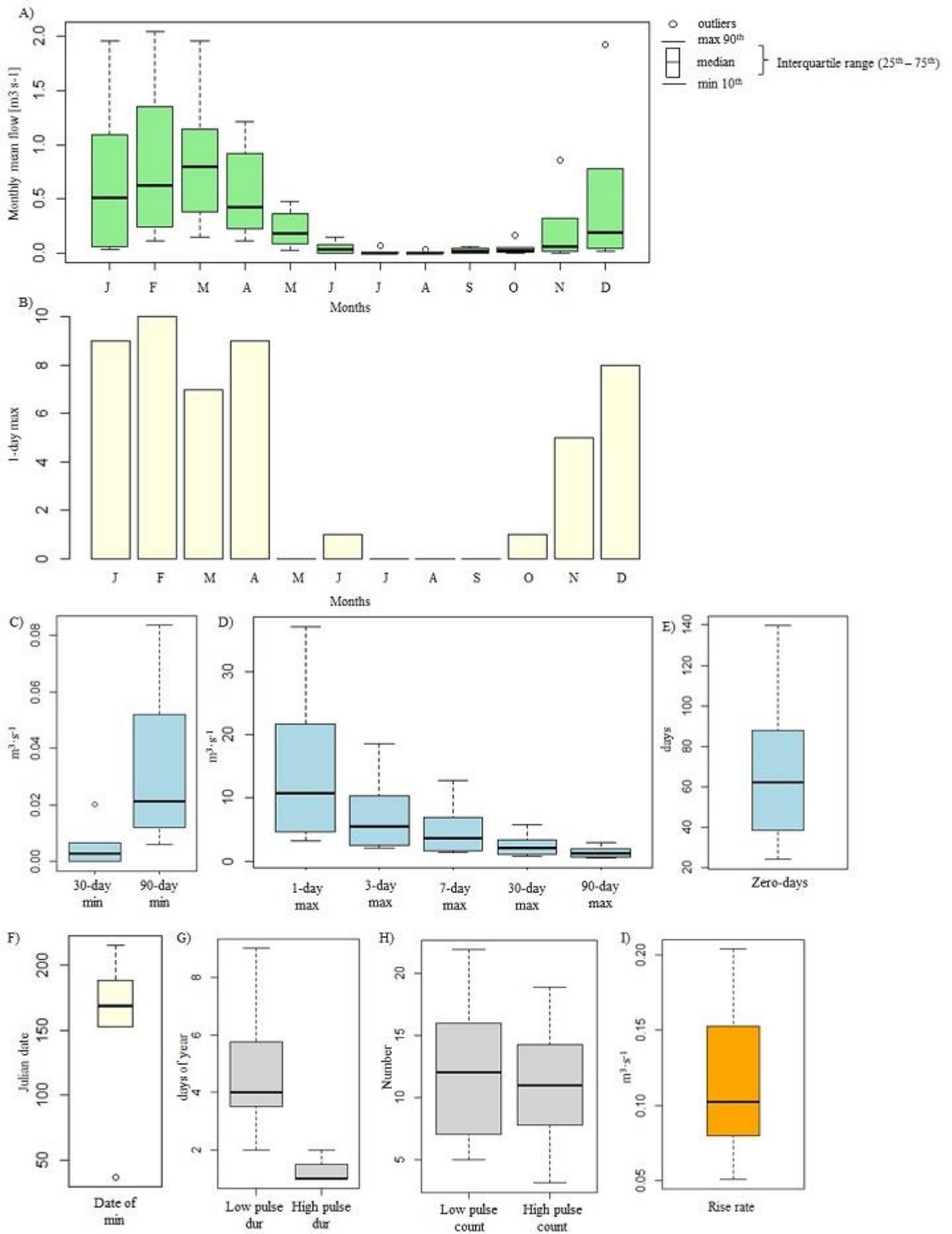
Fig. 4. Boxplot of the selected IHAs computed on un-impacted daily streamflow time series from 1971 to 2020. A) monthly flow; B) number of 1-day max. C) 30-d min and 90-day min; D) 1-day max, 3-day max, 7-day max, 30-day
