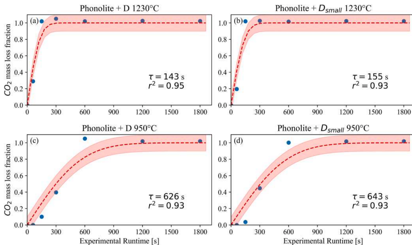
Fig. 6. CO 2 mass loss fraction versus experimental runtime. On the y-axis, a value of 1 describes the maximum theoretical CO 2 loss of the remaining CO 2 (i.e., after the subtraction of initial loss (see Table 3)). Here we compare two different initial clast sizes, resulting in different surface to volume ratios: Fig. 6 a&c are “large” sized ( s/v = 9 \text{ mm}^{-1} ), Fig. 6 b&d are “small” sized ( s/v = 11,33 \text{ mm}^{-1} ). \tau gives the characteristic timescale of decarbonation for each series derived from the fitted curve and the r^2 -value the goodness of the fit.
