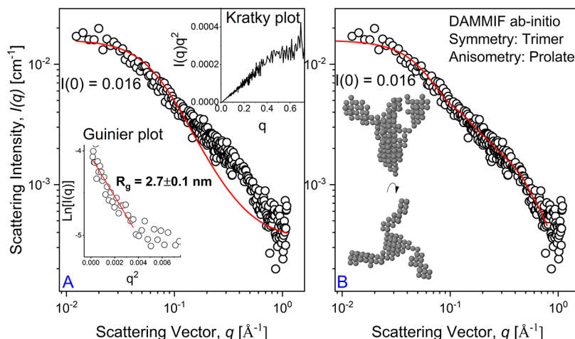
Figure 2. Small-angle X-ray scattering profile of the spike protein of \beta variant of SARS-CoV-2 modeled using the Debye–Gaussian coil model (A) and the ab initio shape determination by DAMMIF (B). Insets in panel (A) are the Guinier plot and the Kratky plot at the bottom and upper part, respectively. Inset in panel (B) is the result of the ab initio simulation of DAMMIF.
