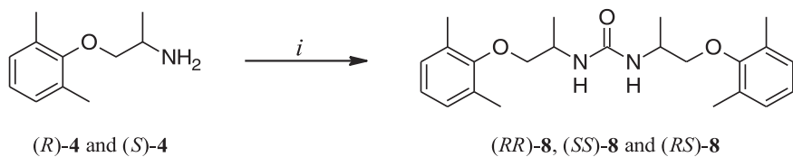
SCHEME 2 Synthesis of (RR)-8, (SS)-8, and (RS)-8. Reagents and conditions: (a) CDI, CH 3 CN, room temp.
