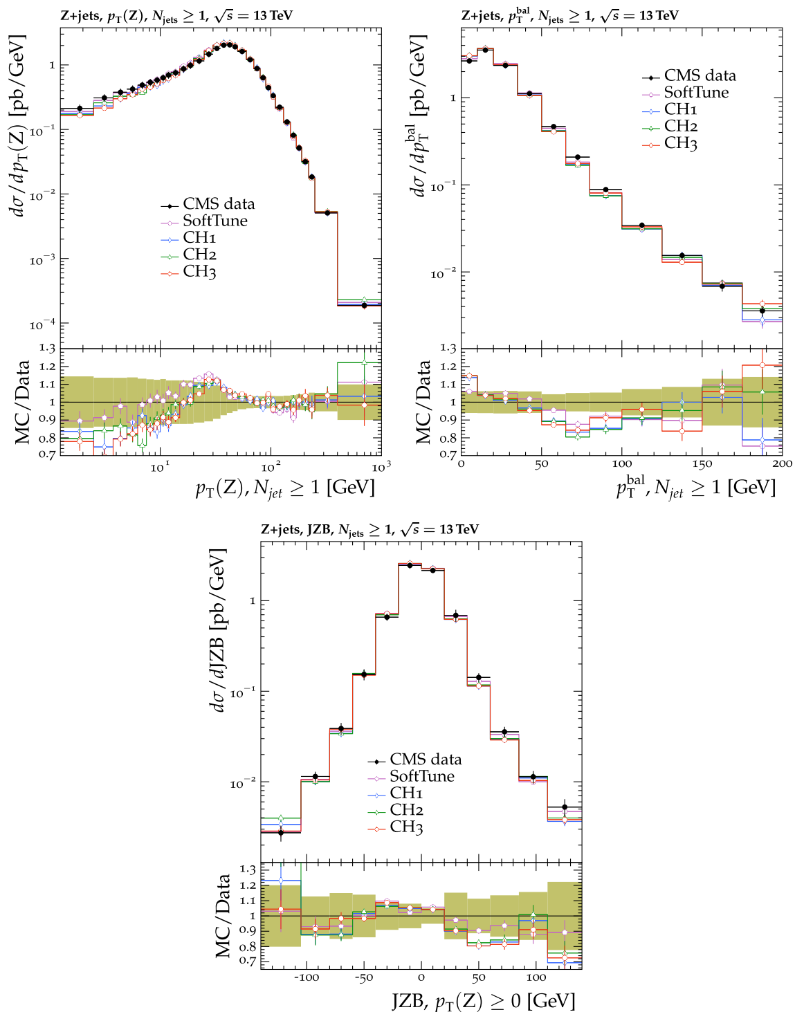
Fig. 19 Differential cross sections as a function of p_T(Z) (upper left), p_T^{\text{bal}} (upper right), and JZB (lower) [46]. CMS Zboson data are compared with the predictions from MADGRAPH5_aMC@NLO + HERWIG 7, with the SoftTune and CH tunes. The coloured band in the ratio plot
